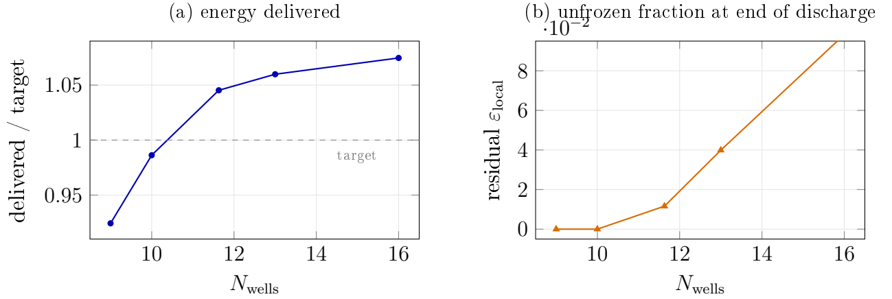
Figure 8: Cyclic steady state against exchanger count; each point is an independent march to convergence. (a) Delivered energy crosses target near N_{\text{wells}} \approx 10.2 , below the latent-only count of 11.63. (b) The diagnostic: the residual melted fraction at end of discharge rises with exchanger count, because each unit is then worked less hard and proportionally less of it refreezes. An inventory-limited store would show the opposite, since a larger store would be proportionally emptier after a fixed discharge. Note that the two panels carry different quantities on similar-looking curves; they are plotted separately for that reason.
