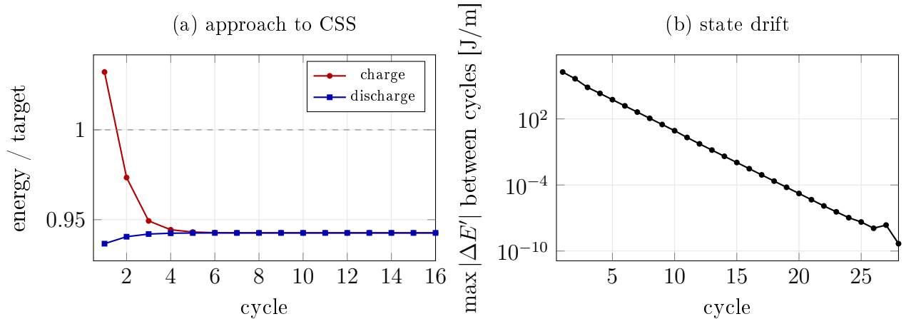
Figure 7: Convergence to cyclic steady state at the latent-only exchanger count. (a) The first cycle is the outlier: it starts from a cold, fully solid store and absorbs more than any later cycle. Charge and discharge converge to the same value, which is Eq. (23) in practice — the two curves become indistinguishable, not merely close. (b) The state drift falls geometrically; the run is stopped at 10^{-9} .
