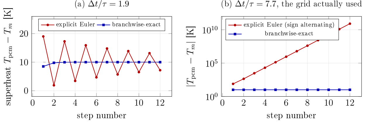
Figure 2: Response of a single segment on the liquid branch, driven by fluid 10 K above T_m with \tau = C_l/K = 1102\text{s} . (a) At \Delta t/\tau = 1.9 explicit Euler oscillates about the equilibrium while remaining bounded. (b) At \Delta t/\tau = 7.7 — the ratio the logarithmic grid of Table 4 actually reaches at the end of a charge — it diverges, alternating in sign and passing 8e10\text{ K} within twelve steps. The branchwise-exact scheme is monotone and correct at every step size, because Eq. (20) cannot overshoot E'_{\text{eq}} .
