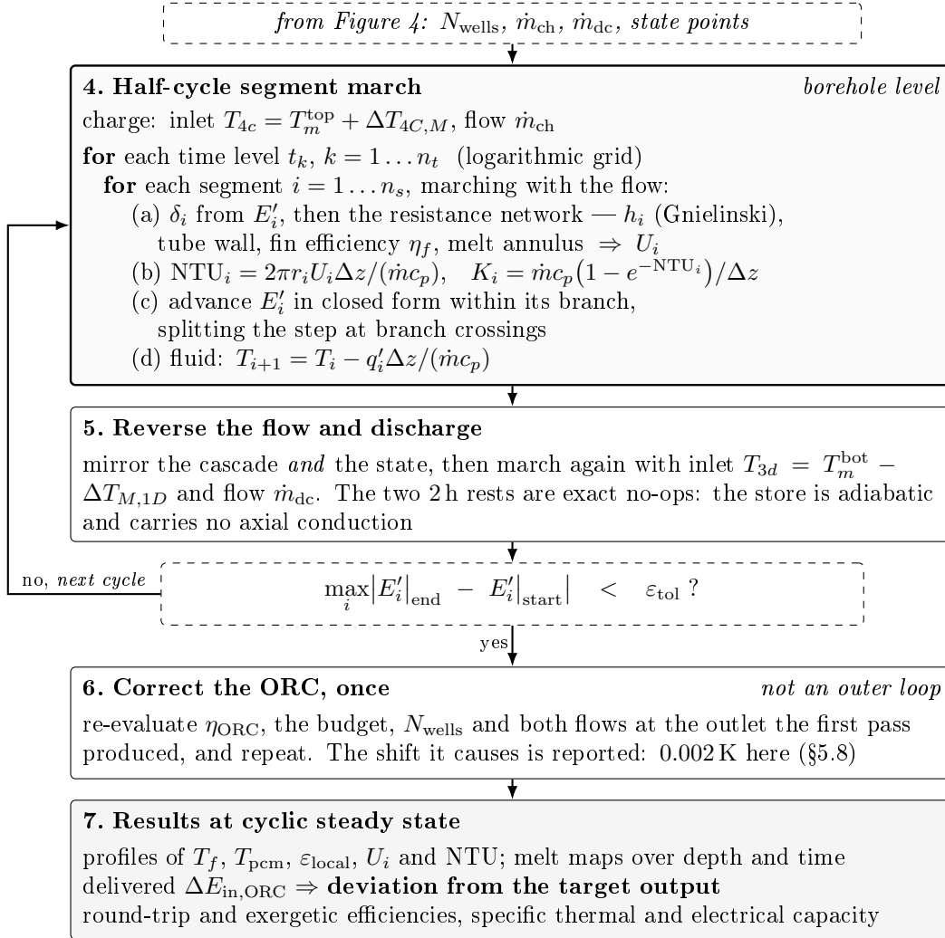
Figure 5: The solution procedure, part 2: the borehole level. Blocks 4 and 5 are the segment march of §2–§4, executed twice per cycle and repeated until the store reproduces its own initial state. That loop is the only iteration in the procedure — block 6 runs once, and is a second evaluation rather than a loop — and no quantity anywhere in Figures 4 and 5 is obtained by root finding, which is a consequence of Eq. (23) rather than a choice (§5.7).
