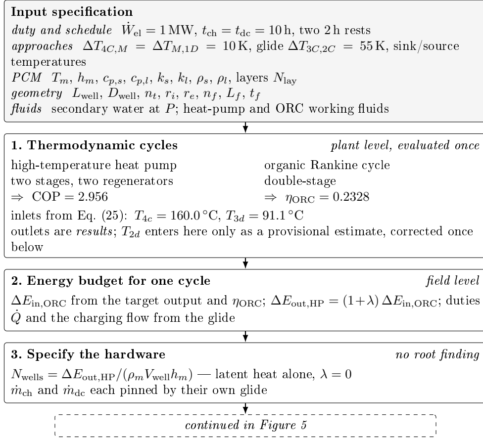
Figure 4: The solution procedure, part 1: the plant and field levels. These blocks are evaluated once, in sequence, and nothing in them is iterated. Their entire output into the rest of the calculation is five secondary-fluid state points, two flow rates and a well count — that is, a fully specified piece of hardware. The borehole model that operates it is Figure 5.
