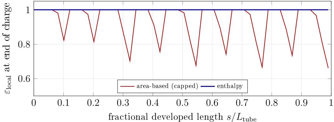
Figure 6: Local melted fraction along the exchanger at end of charge, compared at equal exchanger size with the melted fraction capped in both formulations. The sawtooth in the area-based curve is the cascade: each layer melts fully at its inlet end and incompletely at its outlet end, because a segment that has finished melting continues to draw heat at the full driving difference. Under the enthalpy formulation that segment superheats instead, its demand collapses, and the heat passes downstream — the curve is flat at unity. Spread falls from 0.405 to 0.000 (Table 5).
