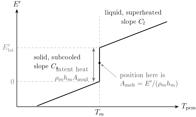
Figure 1: The constitutive curve, Eq. (2). Read as E'(T) it is multivalued at T_m , which is why temperature cannot serve as the state. Read as T(E') — the direction used here — it is single-valued everywhere, and position along the vertical segment is the melted fraction.
