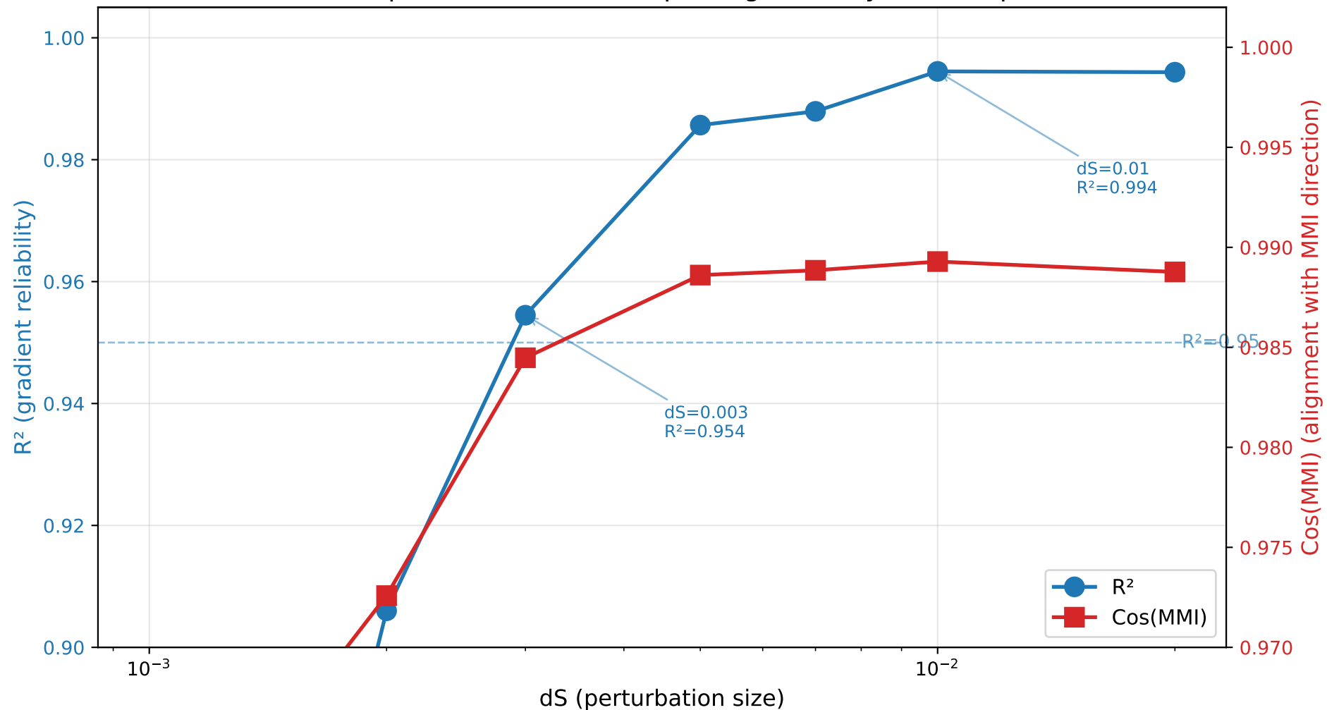
Gradient Quality vs Perturbation Size (dS) max10 experiments (10x max pooling), n=3 symmetric point
