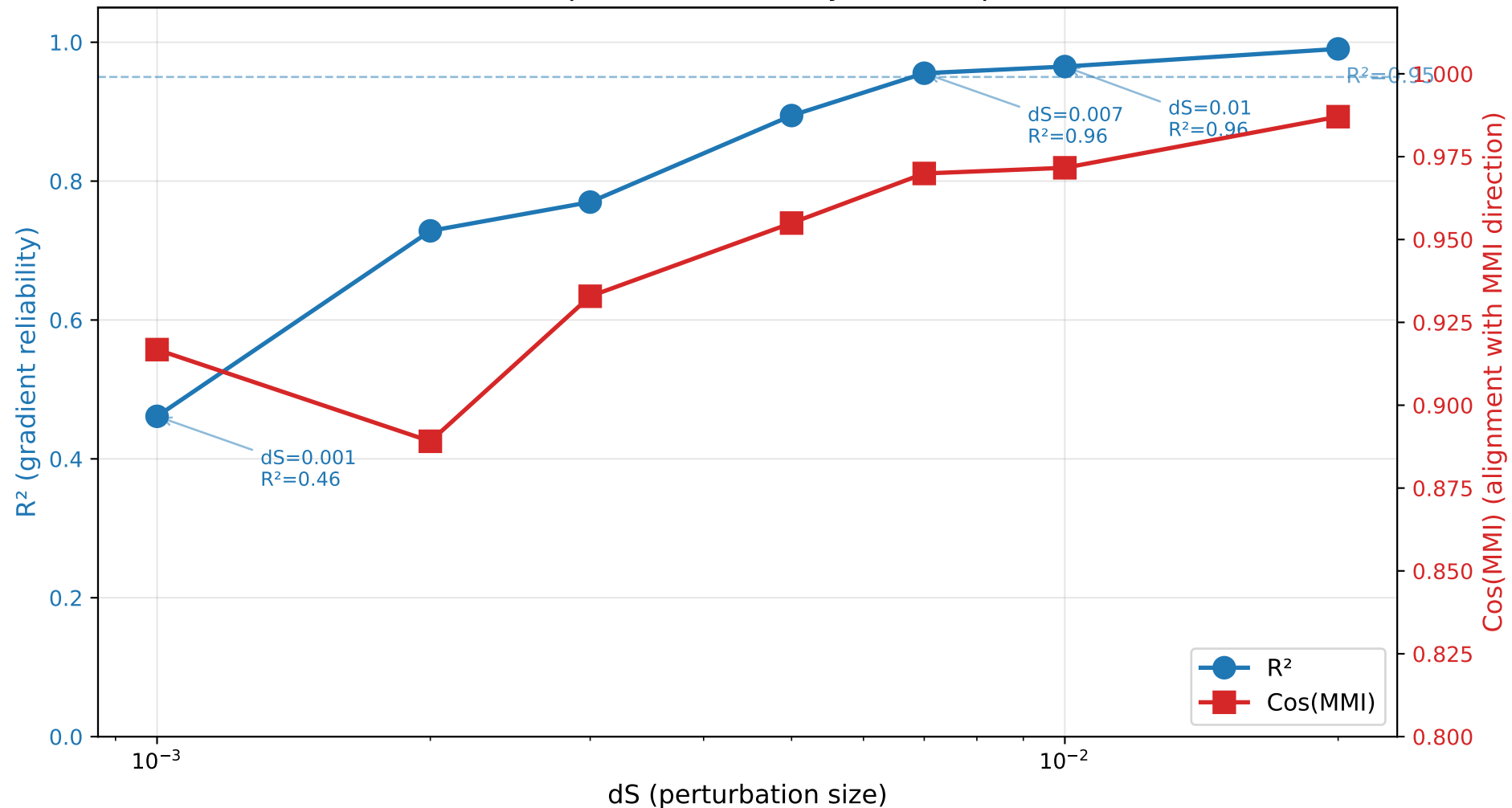
Gradient Quality vs Perturbation Size (dS) max1 experiments, n=3 symmetric point
