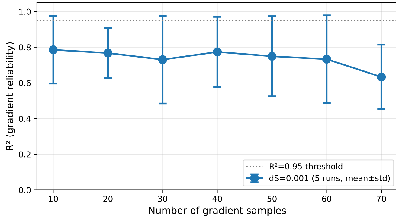
Gradient Reliability ( R^2 ) vs Sample Size dS=0.001
