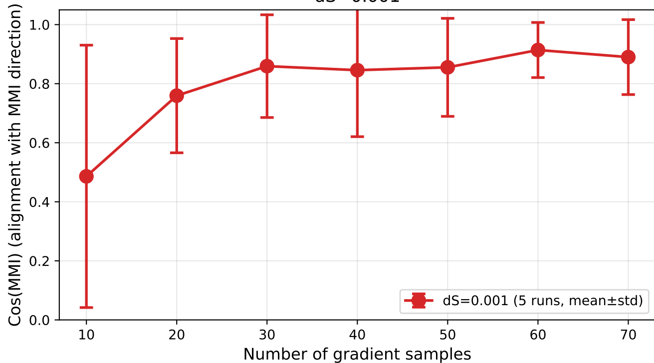
MMI Alignment (Cosine) vs Sample Size dS=0.001
