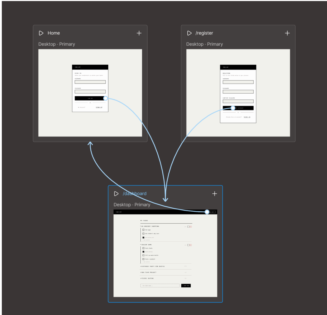
Figure 9: Screen navigation — home, register, and dashboard
