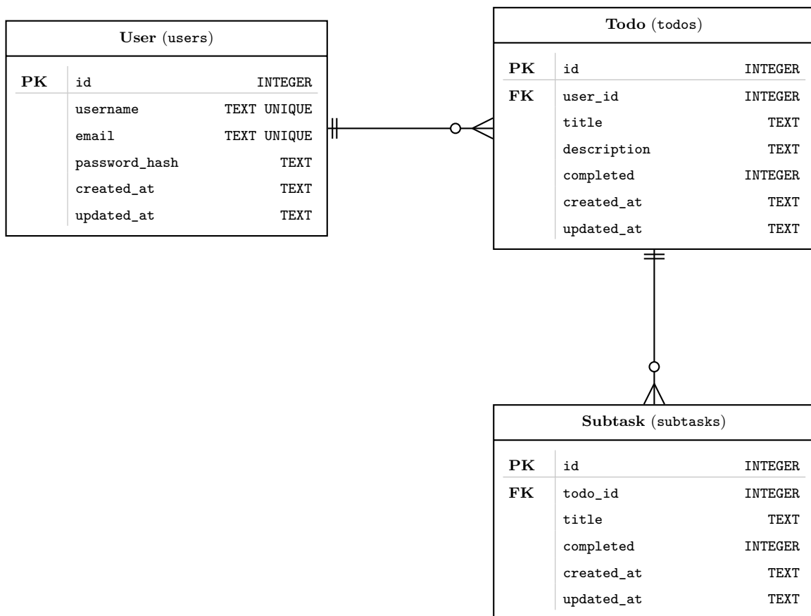
Figure 1: Crow's Foot ERD
