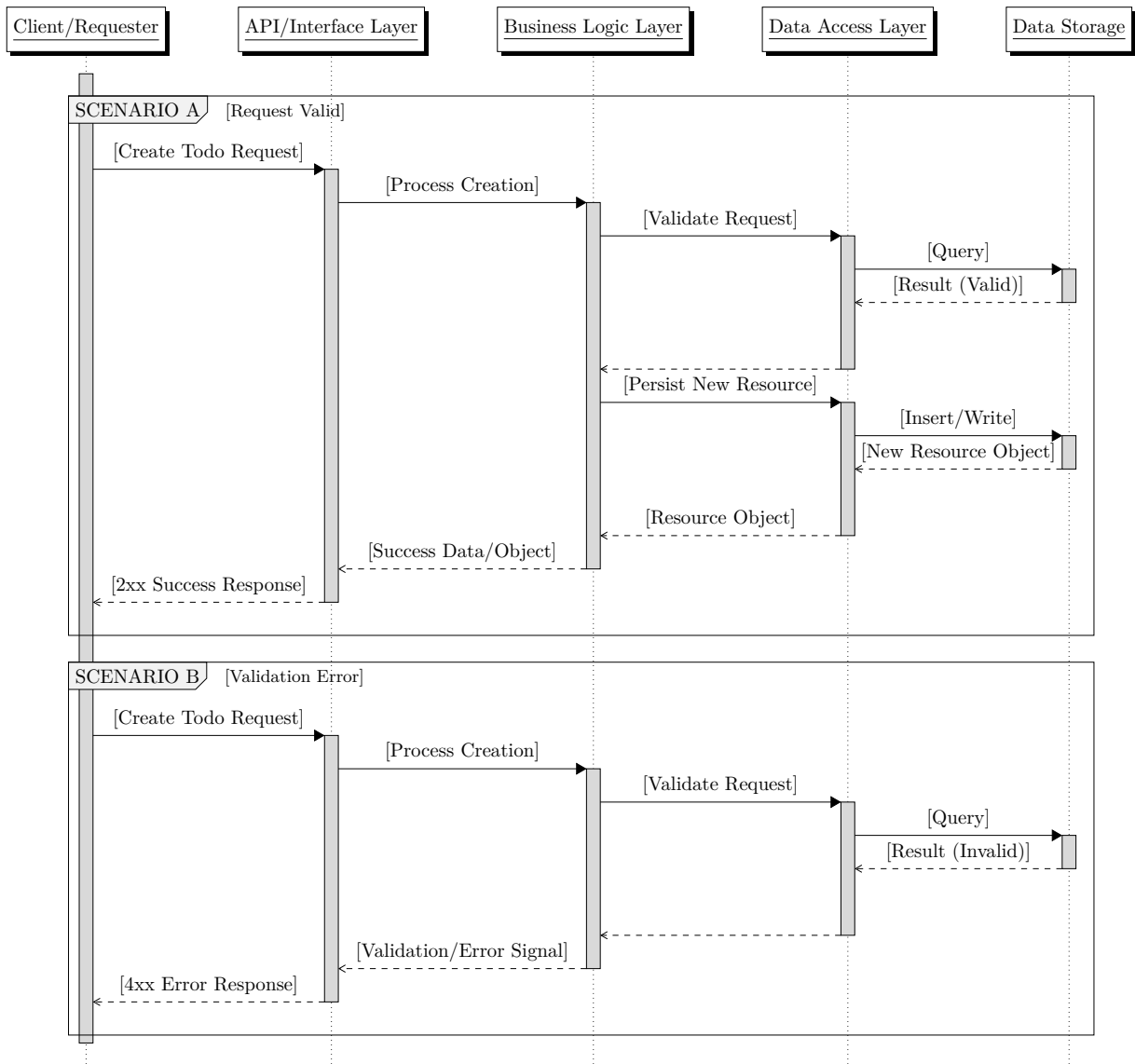
Figure 3: Task management — POST /api/todos
