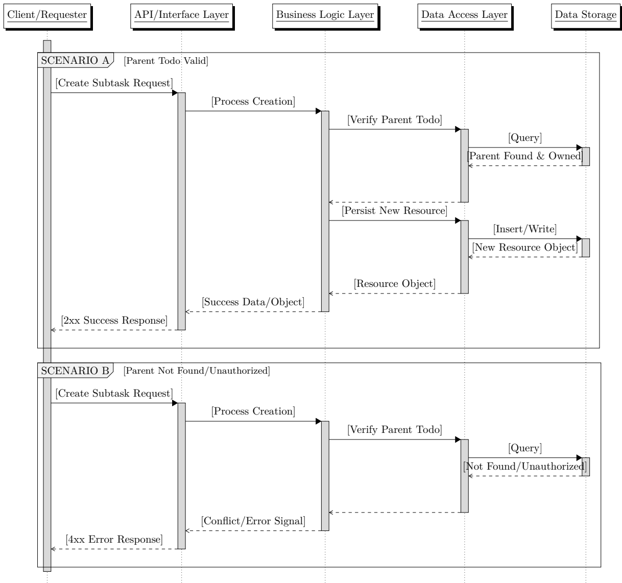
Figure 4: Subtask organization — POST /api/todos/{id}/{subtask}
