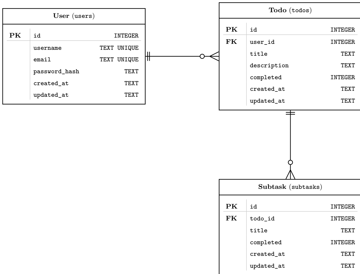
Figure 5: Crow's Foot ERD
