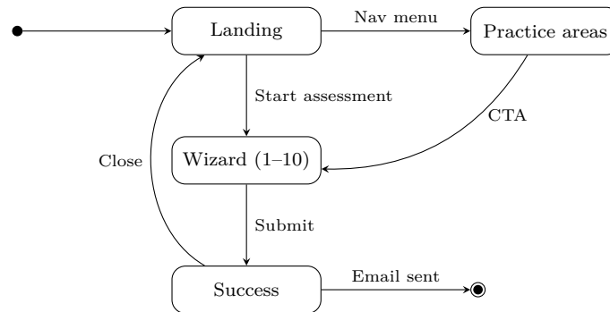
Figure 3: UML Activity Diagram - UI flow
