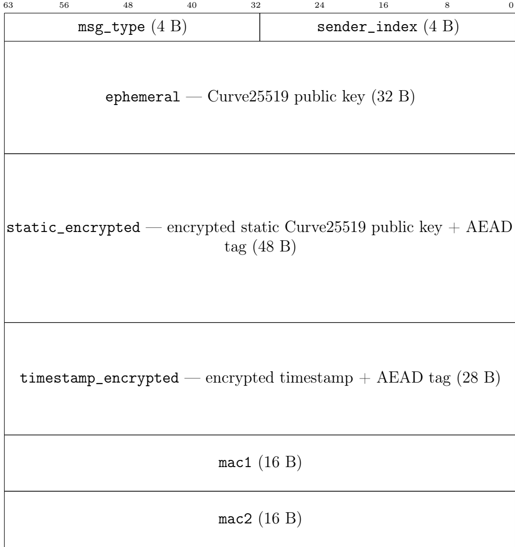
Figure 4: WireGuard handshake initiation message (148 bytes total)
