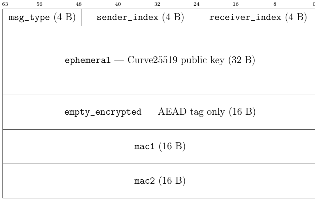
Figure 5: WireGuard handshake response message (92 bytes total)
