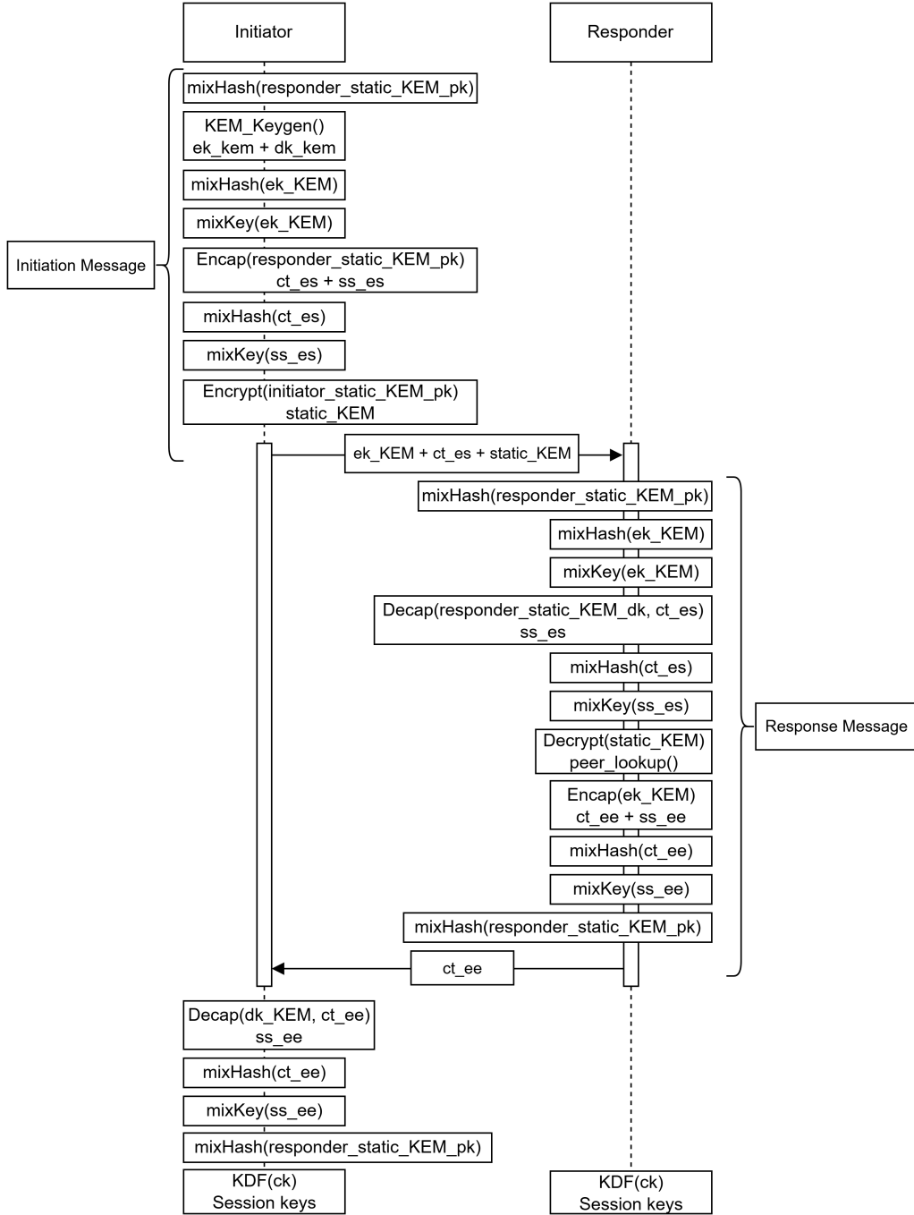
Figure 6: Flow diagram of the pure-KEM handshake. All DH operations from the classical handshake are replaced by KEM encapsulation and decapsulation operations.
