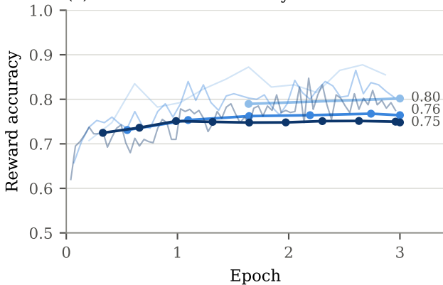
(c) DPO: reward accuracy
