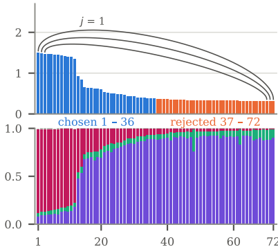
Missing or incorrect factual knowledge context 150, n = 72 , u = (0.28, 0, 0.47, 1.67)
