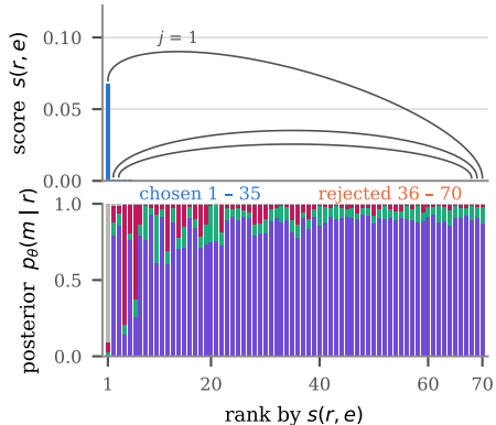
Misunderstanding of the question context 331, n = 70 , u = (0, 0.07, 0, 0)
