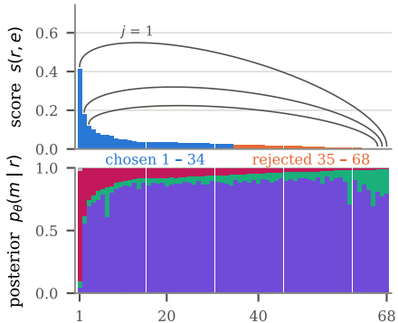
Missing or extra quantity context 635, n = 68 , u = (0, 0.05, 0, 0.47)
