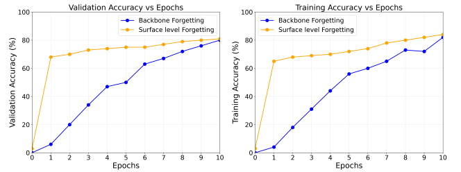
Fig. 5. CU recovers gradually (genuine) vs. rapid head-masking (superficial).
