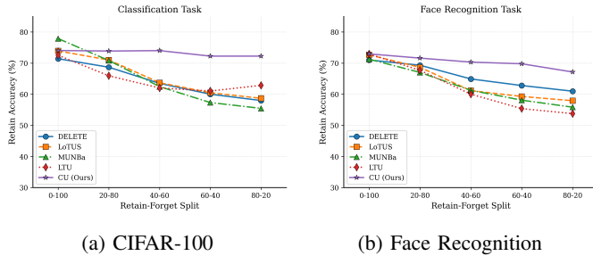
Fig. 3. Retain accuracy across sequential unlearning cycles. Existing methods degrade progressively while CU maintains stable performance on both benchmarks.
