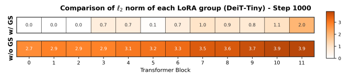
Fig. 2. \ell_2 norm per block. Localized regularization concentrates updates in specific blocks.
