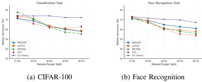
Fig. 3. Sequential-cycle retain accuracy; baselines degrade, CU stable.
