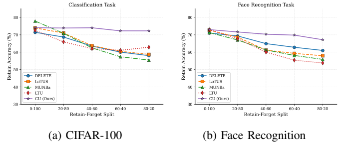
Fig. 3. Retain accuracy across sequential unlearning cycles. Existing methods degrade progressively while CU maintains stable performance on both benchmarks.
