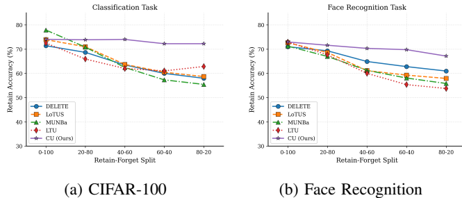
Fig. 6. Retain accuracy across sequential unlearning cycles. Existing methods degrade progressively while CU maintains stable performance on both benchmarks.
