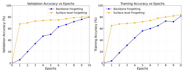
Fig. 4. Backbone vs surface-level unlearning. CU recovers gradually (genuine forgetting) while head-masking recovers rapidly (superficial).
