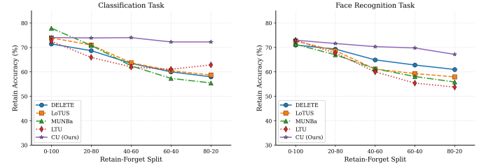
(a) CIFAR-100
