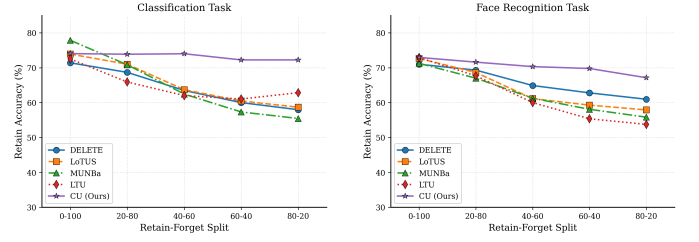
(a) CIFAR-100
