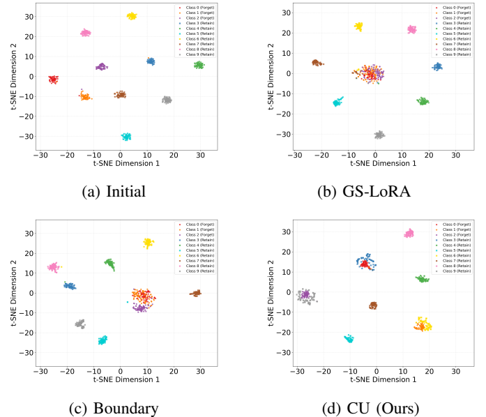
Fig. 1. t-SNE embeddings: baselines collapse to one point; CU distributes to nearest boundaries.
