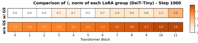
Fig. 2. \ell_2 norm per block: updates concentrate in a few blocks.
