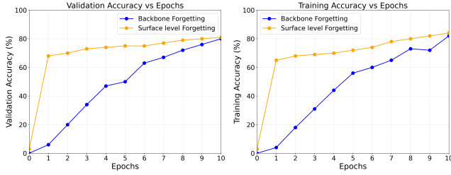
Fig. 5. CU recovers gradually (genuine forgetting) vs. rapid head-masking recovery (superficial).
