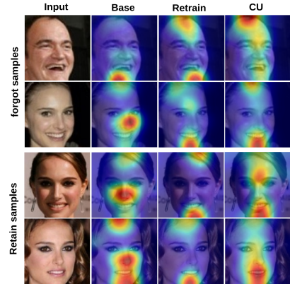
Fig. 4. Attention maps on forget and retain samples (input, base, retrained, CU). Retrained/CU models disperse attention off-face only for forget identities, confirming surgical removal.
