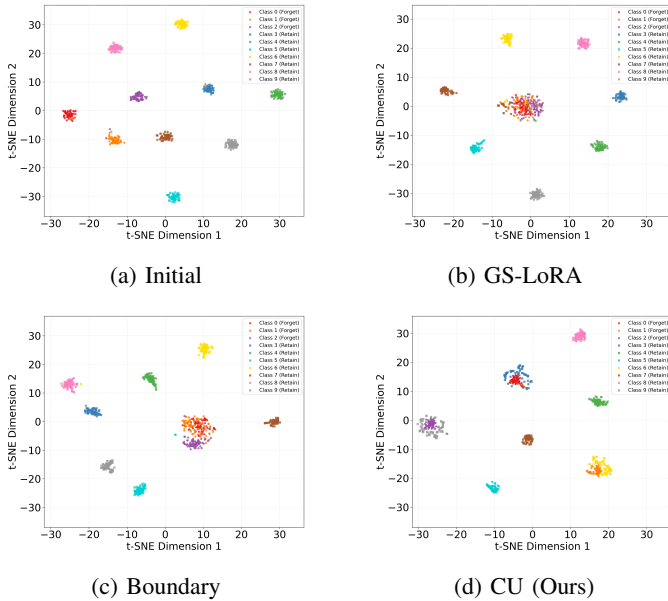
Fig. 1. t-SNE visualization. Baselines collapse to single point while proposed CU method distributes to nearest boundaries thus achieving faster convergence.
