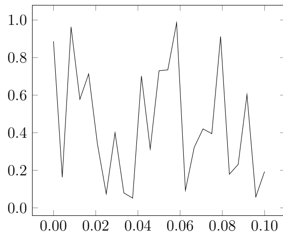
Figure 3.1: Figure caption.
