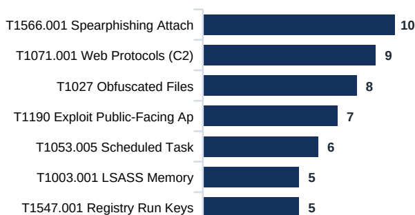
Most common ATT&CK techniques across APT profiles
