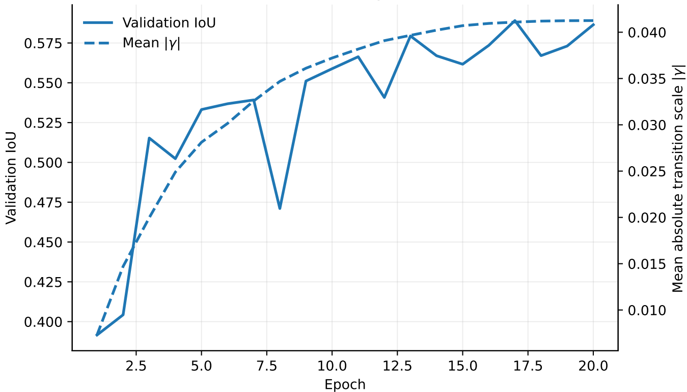
Seed 2026: Transition Strength vs Validation IoU
