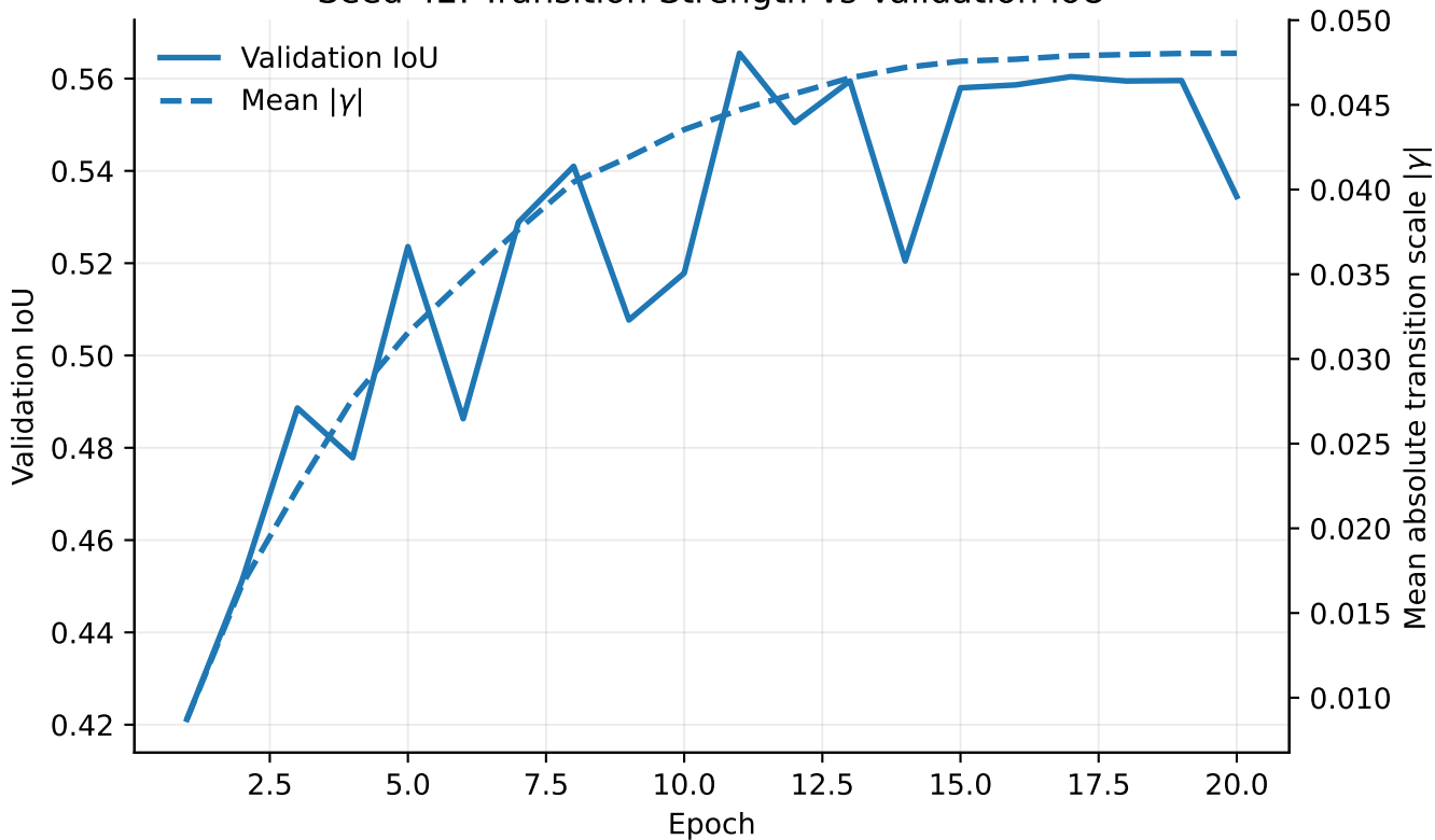
Seed 42: Transition Strength vs Validation IoU
