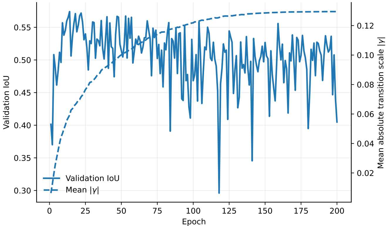
TCSF v3.1, 200 epochs: Transition Strength vs Validation IoU
