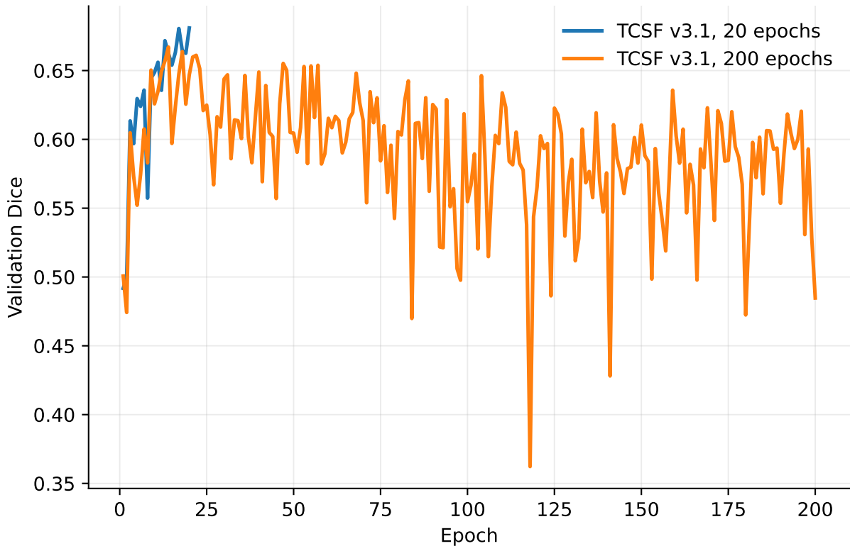
Validation Dice
