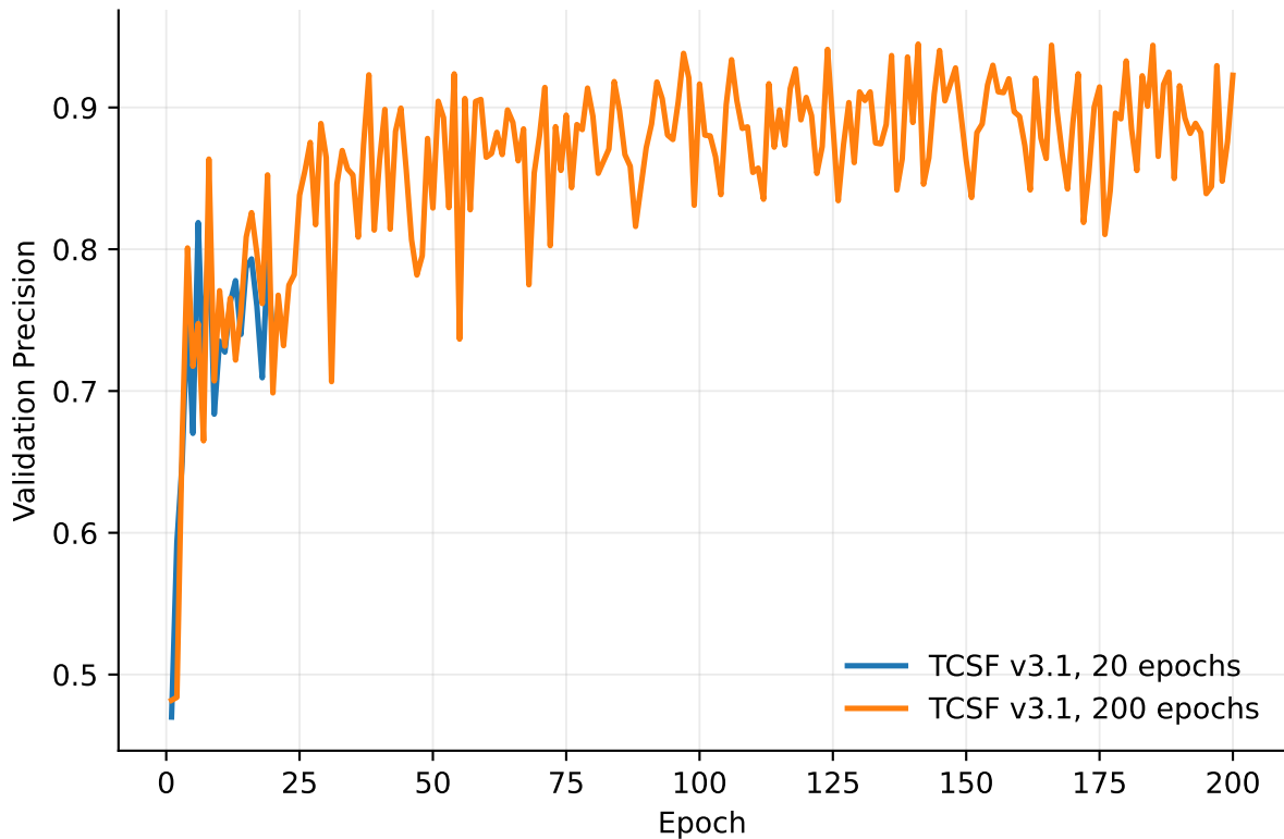
Validation Precision
