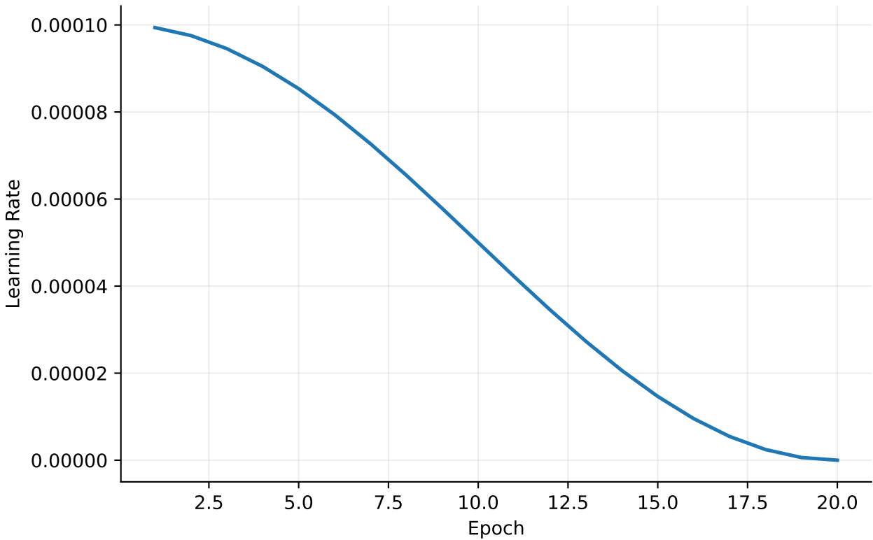
Learning-Rate Schedule
