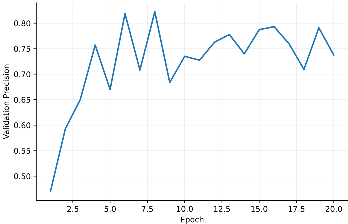
Validation Precision
