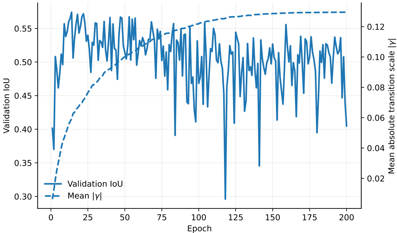
TCSF v3.1: Transition Strength vs Validation IoU
