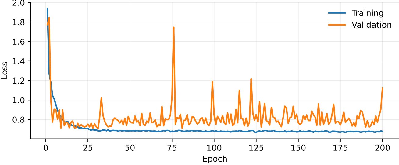
Swin-UNet
