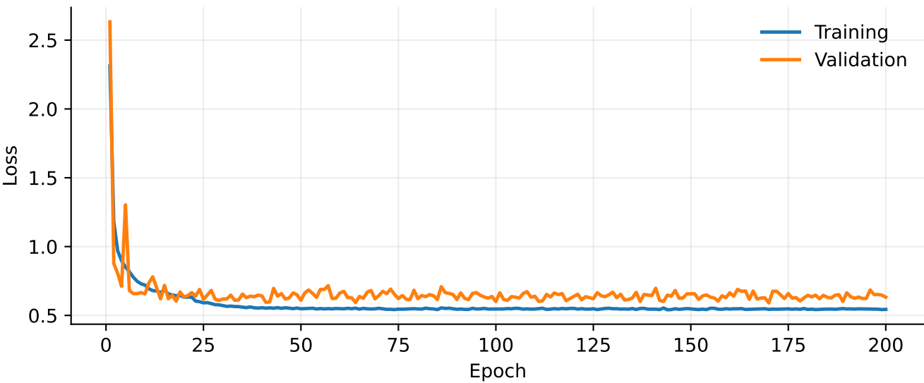
DeepLabV3+
