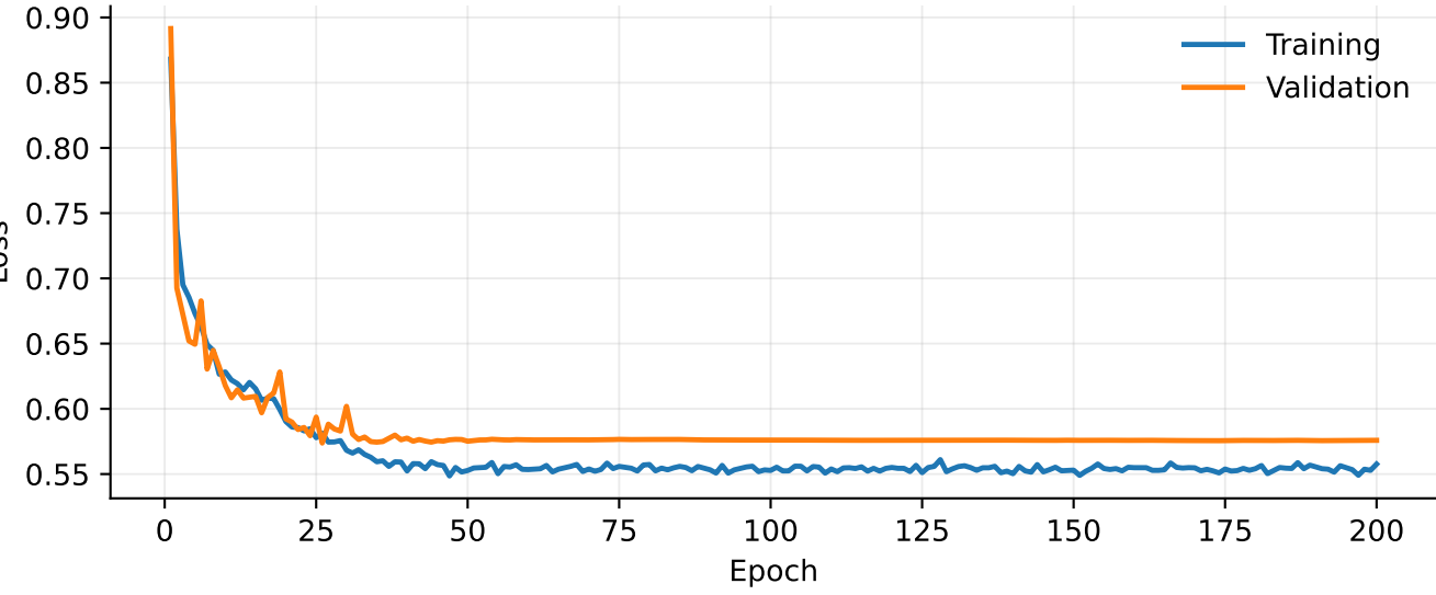
Vision Mamba
