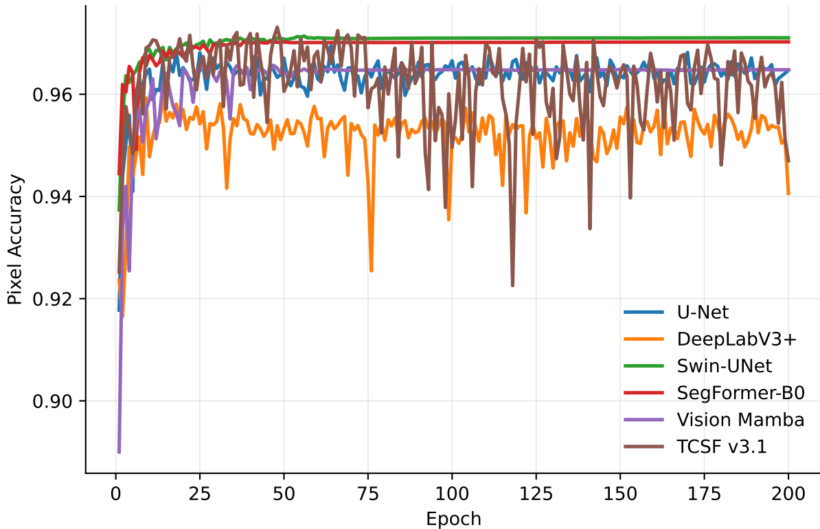
Validation Pixel Accuracy
