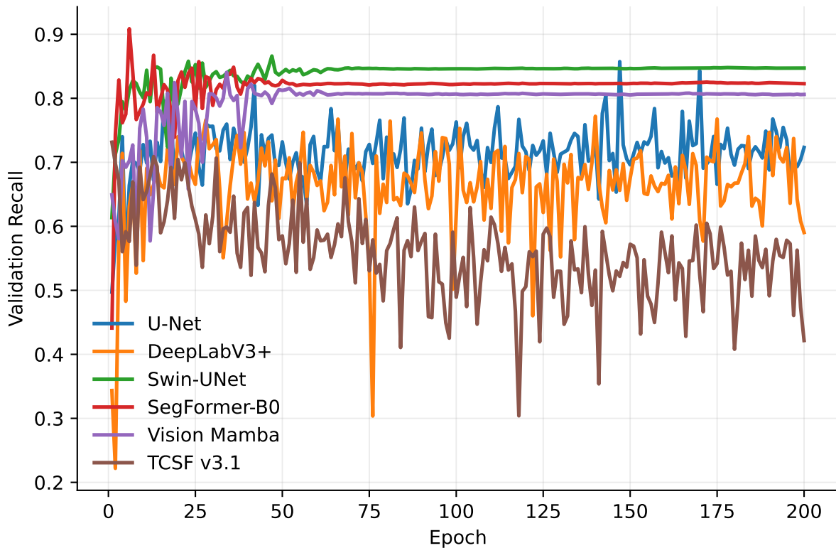
Validation Recall
