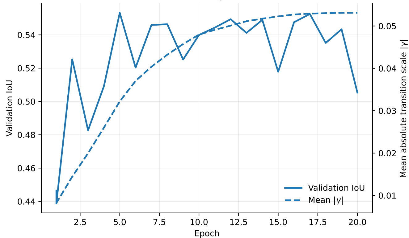
RU-TCSF: Transition Strength vs Validation IoU
