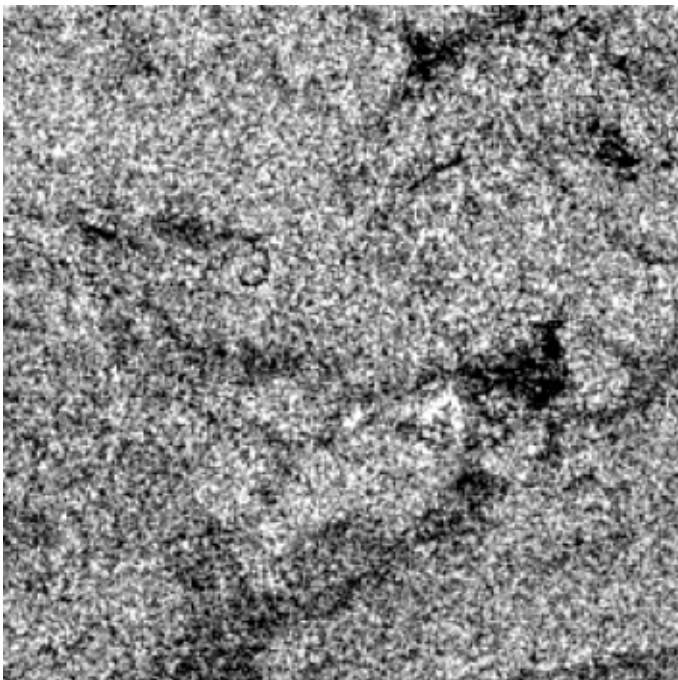
U-Net IoU: 0.489
