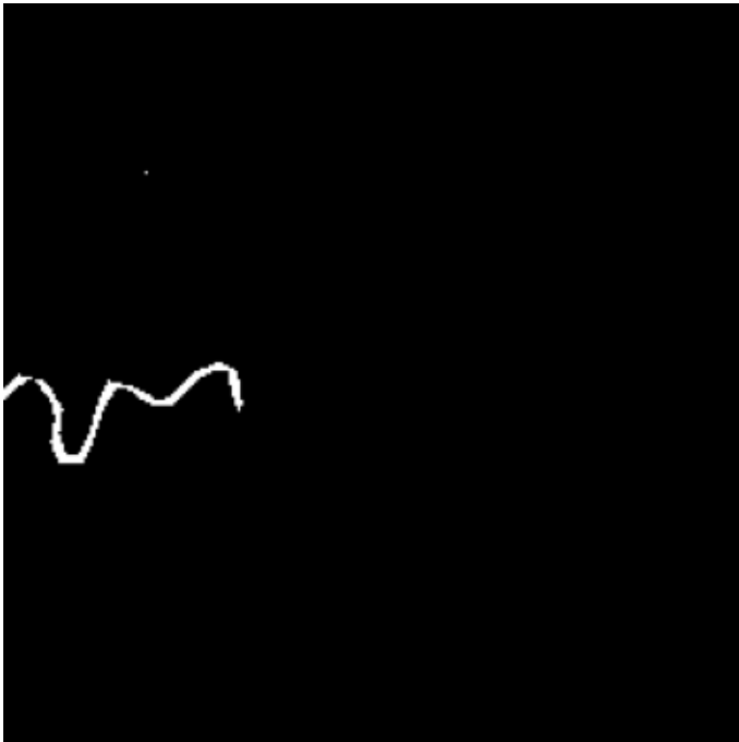
Swin-UNet IoU: 0.000
