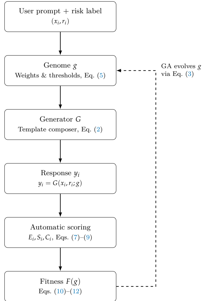
Figure 1. Overview of the EvoRiri response-generation and optimization pipeline, with the governing equation shown for each stage. A genome g (Eq. (5)) parametrizes the template-based generator G (Eq. (2)), which produces a response y_i for each prompt-risk pair (x_i, r_i) . Automatic scoring (Eqs. (7)–(9)) yields the per-example and global fitness (Eqs. (10)–(12)), which the genetic algorithm uses to evolve the genome via the objective in Eq. (3).
