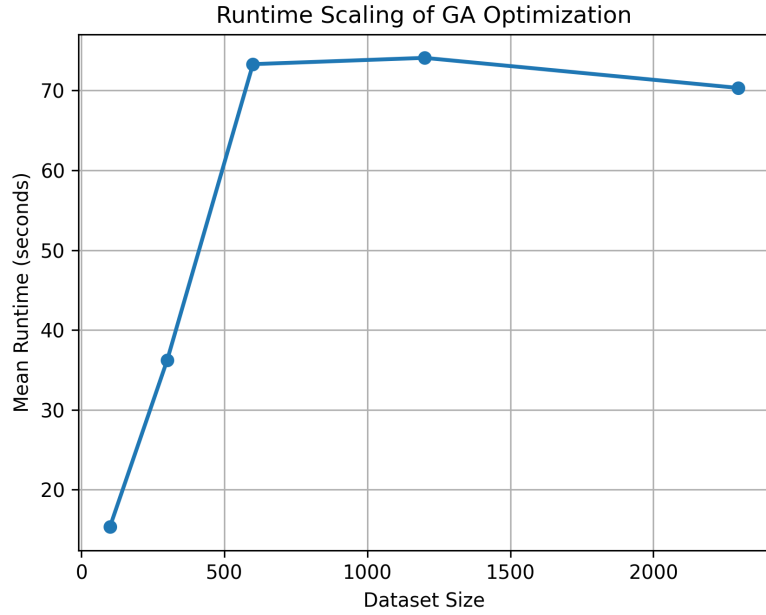
Figure 9. Runtime scaling of GA optimisation with dataset size. Mean runtime increases from approximately 15 seconds at N = 100 to a plateau of 70–75 seconds beyond N = 600 , confirming that the evaluation subset cap of |\mathcal{I}| = 600 dominates runtime independently of total dataset size.
