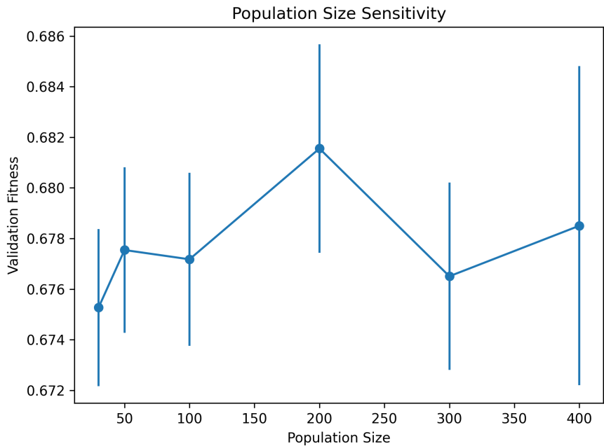
Figure 3. Population size sensitivity analysis. Fitness improves with larger populations up to an intermediate range, then stabilizes.
