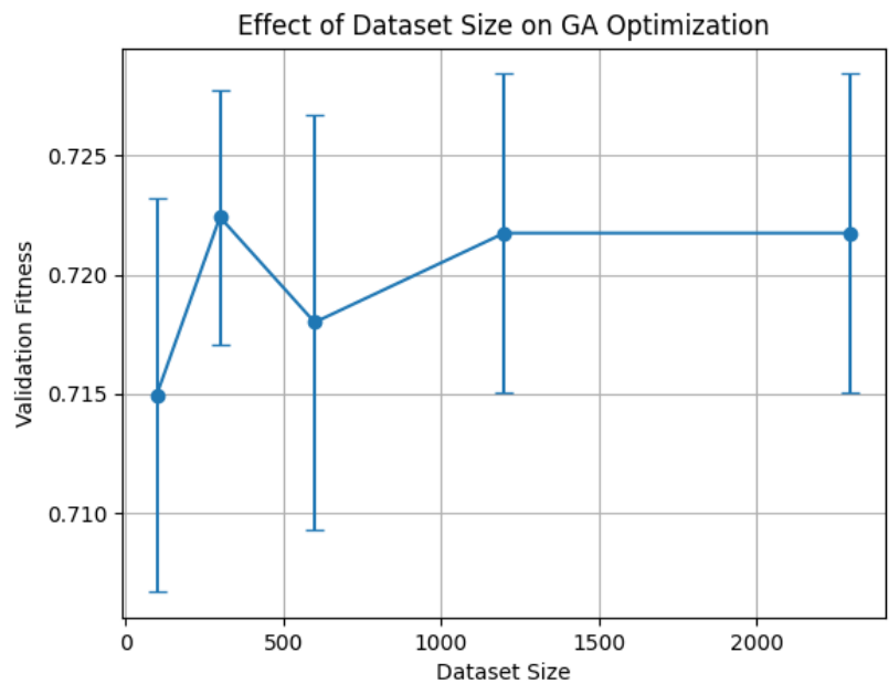
Figure 2. Effect of dataset size on validation fitness. Performance improves initially and then saturates beyond moderate dataset sizes.
