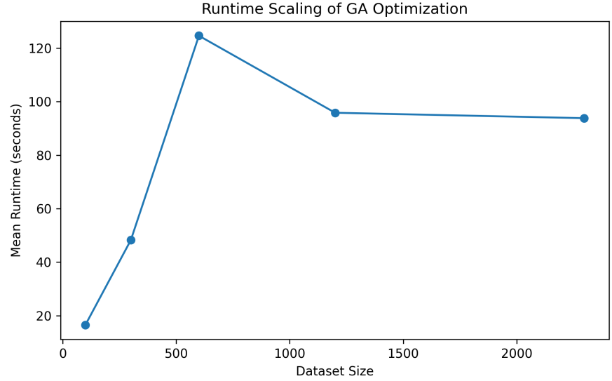
Figure 9. Runtime scaling of GA optimisation with dataset size. Mean runtime increases from approximately 16.5 seconds at N = 100 to a peak of 124.6 seconds at N = 600 , then decreases to approximately 94–96 seconds for N \geq 1200 rather than remaining flat, a pattern we attribute to system-level timing variability on non-dedicated hardware rather than to the algorithm’s computational complexity, which is fixed once the evaluation subset saturates at |\mathcal{I}| = 600 .
