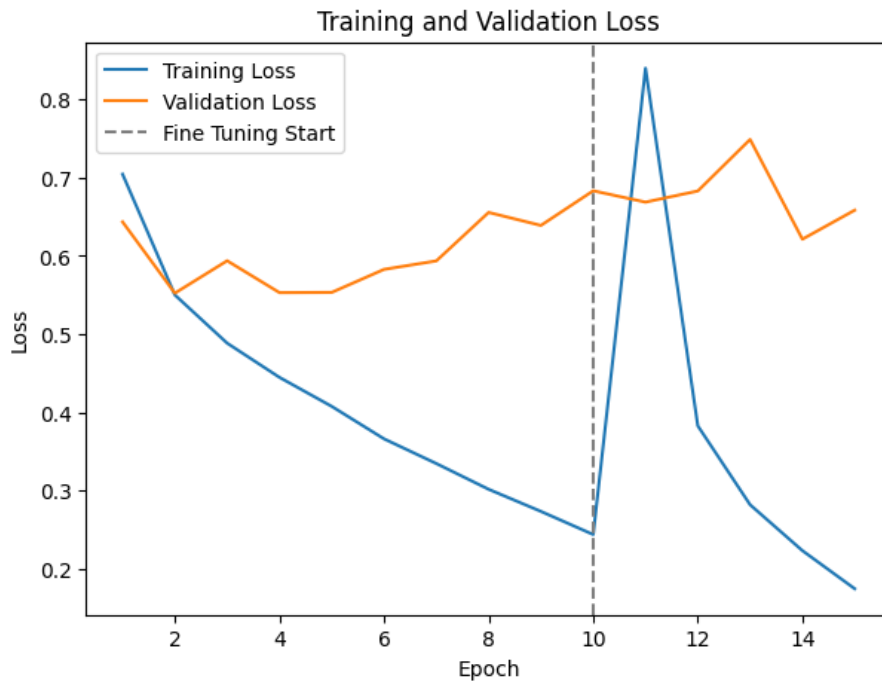
Figure 5: Training and Validation Loss
