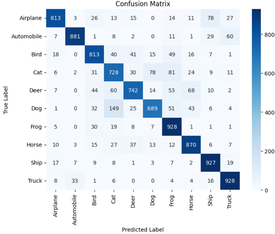
Figure 6: Confusion Matrix
