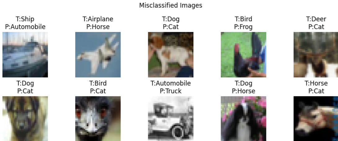
Figure 7: Misclassified Images
