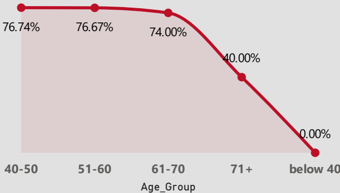
Survival_Rate by Age_Group
