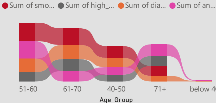
Health Condition Impact Dashboard: Smoking, BP, Anemia & Diabetes
