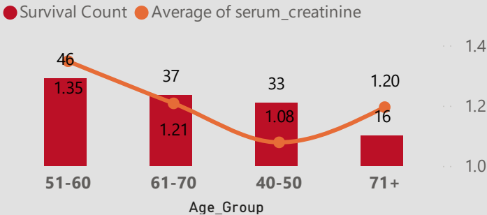
Survival Count and Average Serum Creatinine By Age Group
