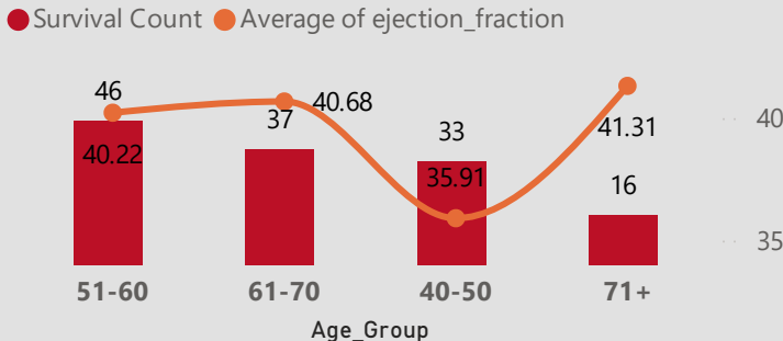
Survival Count and Average Ejection Fraction By Age Group
