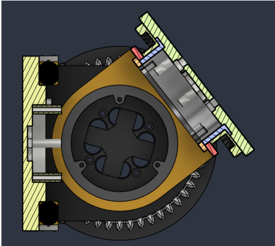
Figure 5: Tilted sectional view of the module CAD design.
