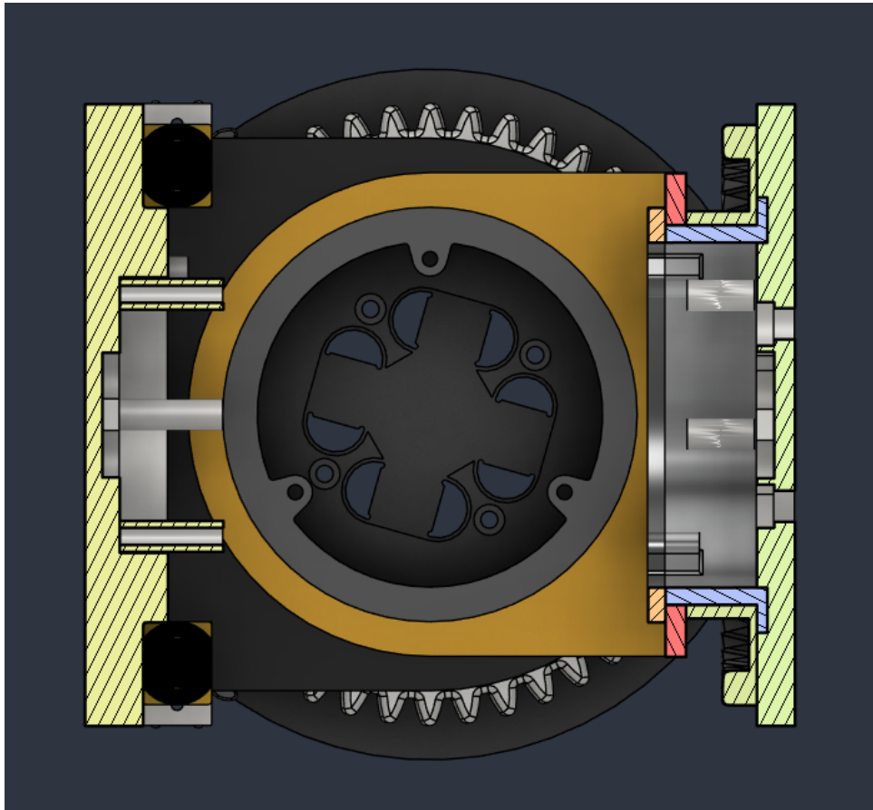
Figure 8: Interior view of the wheel and drivetrain assembly.
