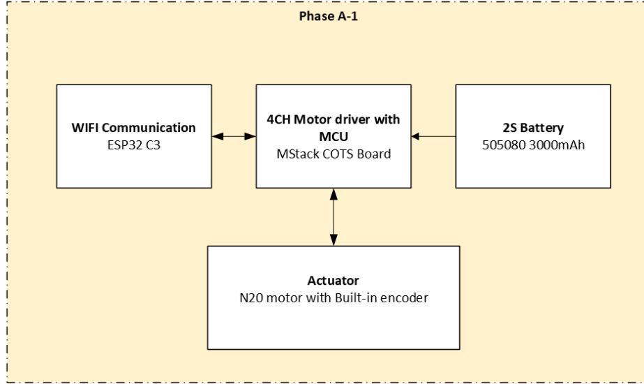
Figure 10: Phase A-1 electronics block diagram.
