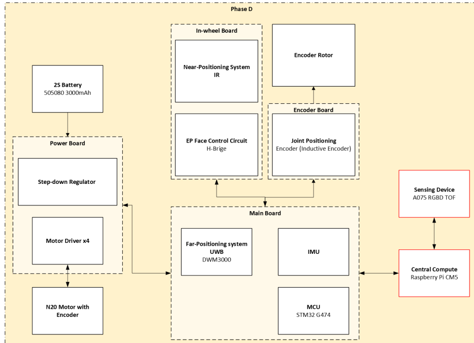
Figure 14: Phase D electronics block diagram.
