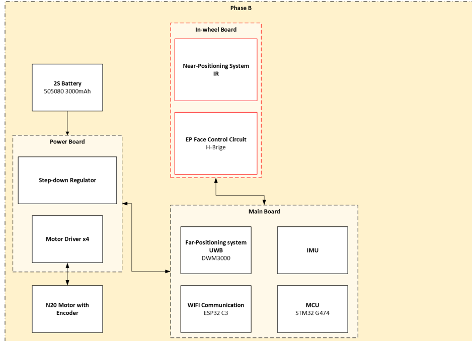
Figure 12: Phase B electronics block diagram.
