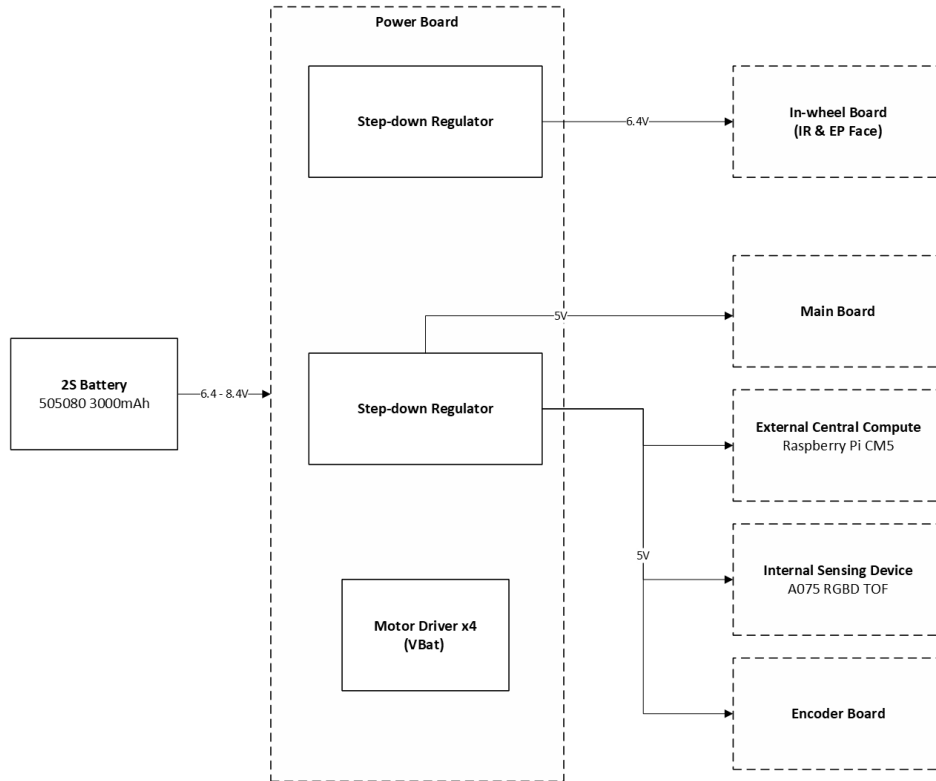
Figure 17: Power distribution block diagram.
