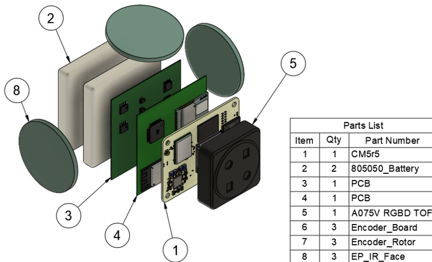
Figure 16: Electronics packaging CAD, exploded view.
