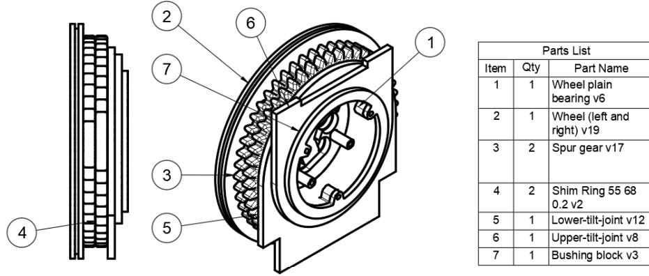
Figure 19: Shaft and bearing component arrangement.
