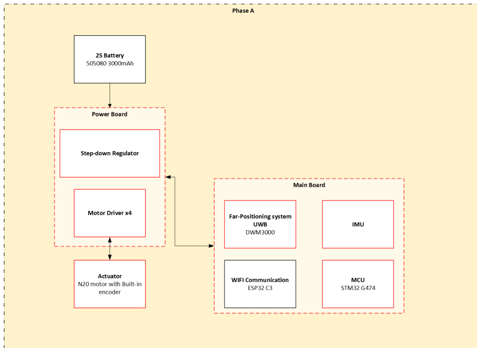
Figure 11: Phase A electronics block diagram.
