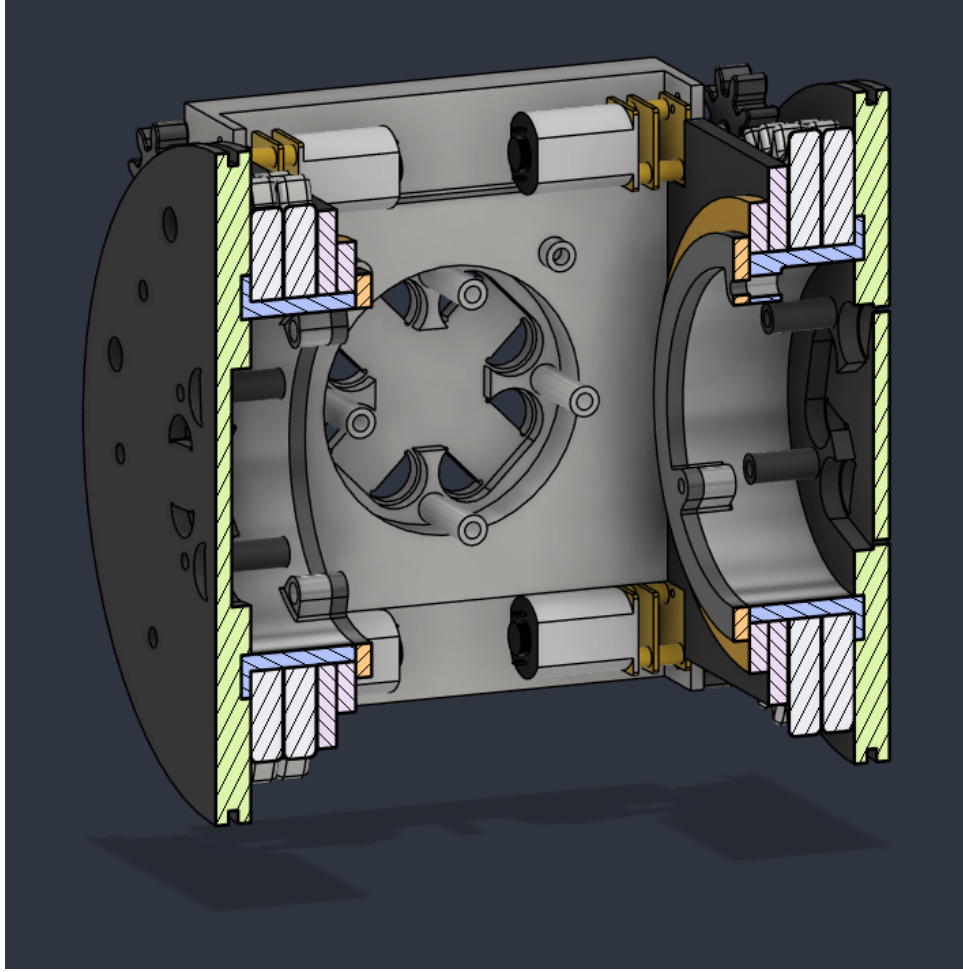
Figure 18: Interior view of the rectangular magnet housing.
