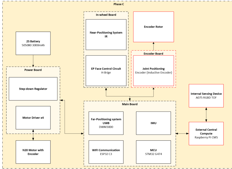
Figure 13: Phase C electronics block diagram.
