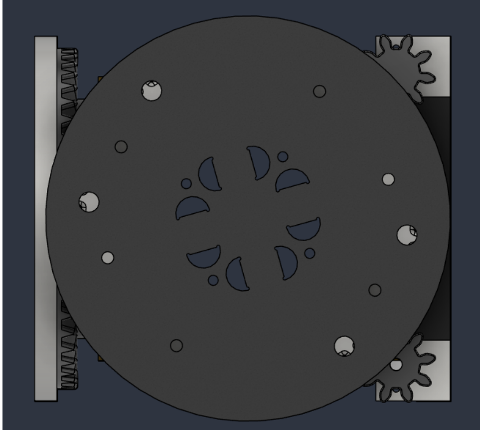
Figure 9: Exterior view of the wheel and module assembly.
