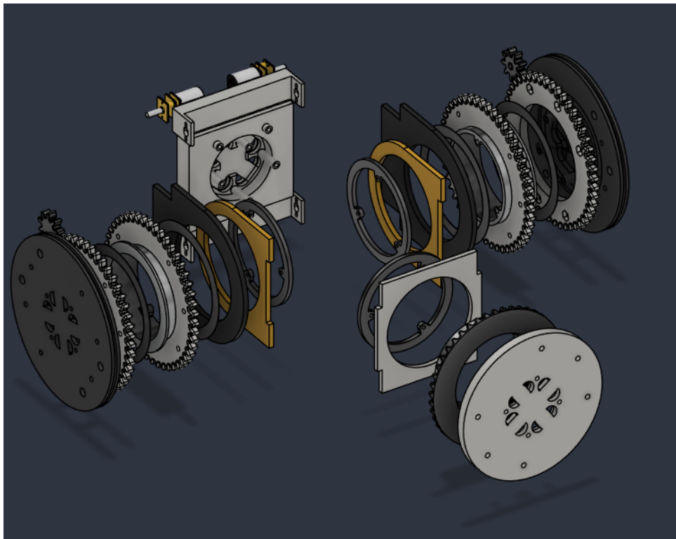
Figure 1: Exploded view of the module CAD design.
