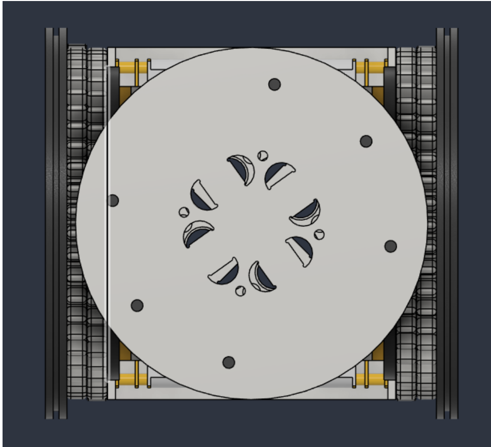
Figure 2: Front view of the module CAD design.
