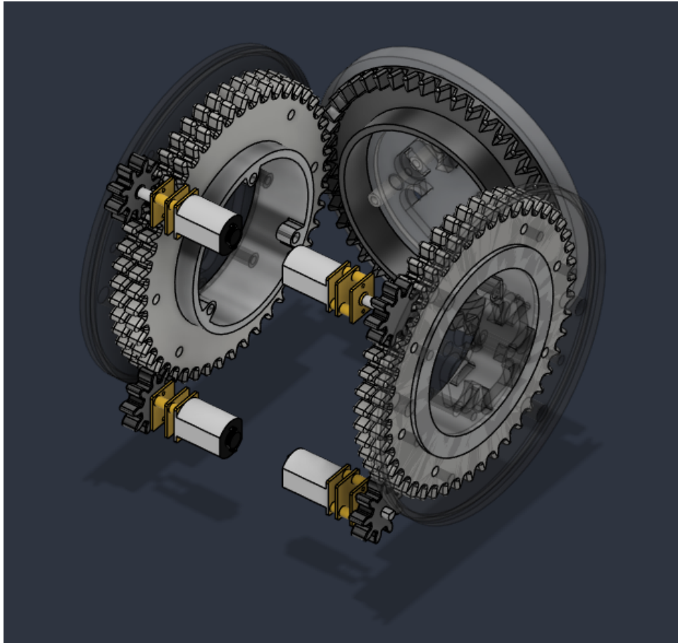
Figure 6: CAD view of the gear train and motor arrangement.
