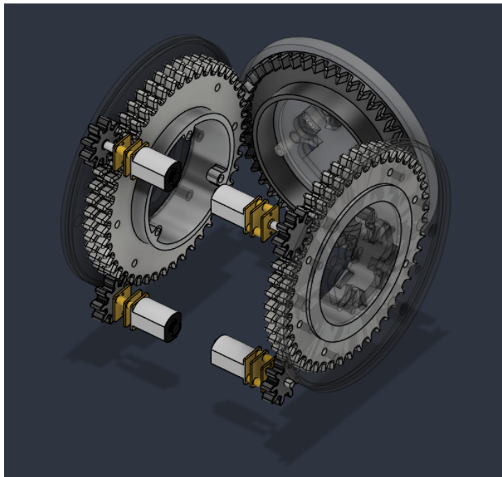
Figure 5: CAD view of the gear train and motor arrangement.
