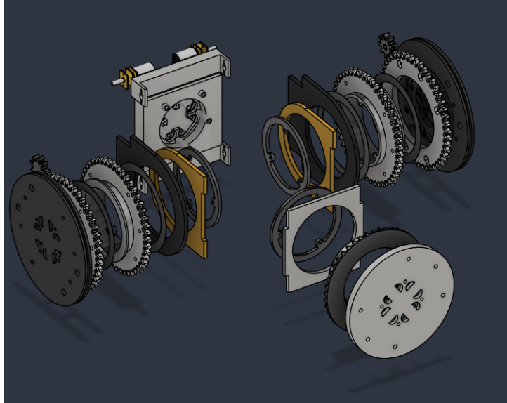
Figure 3: Exploded view of the module.
