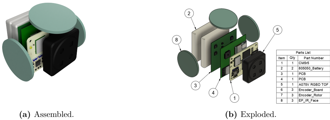
Figure 10: Electronics packaging.
