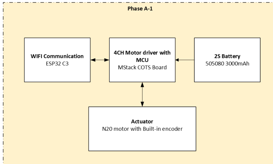
Figure 7: Phase A-1 electronics block diagram.
