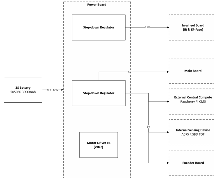
Figure 11: Power distribution block diagram.
