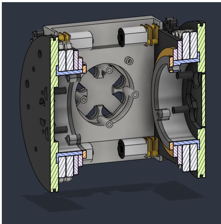
Figure 13: Interior view of the rectangular magnet housing.
