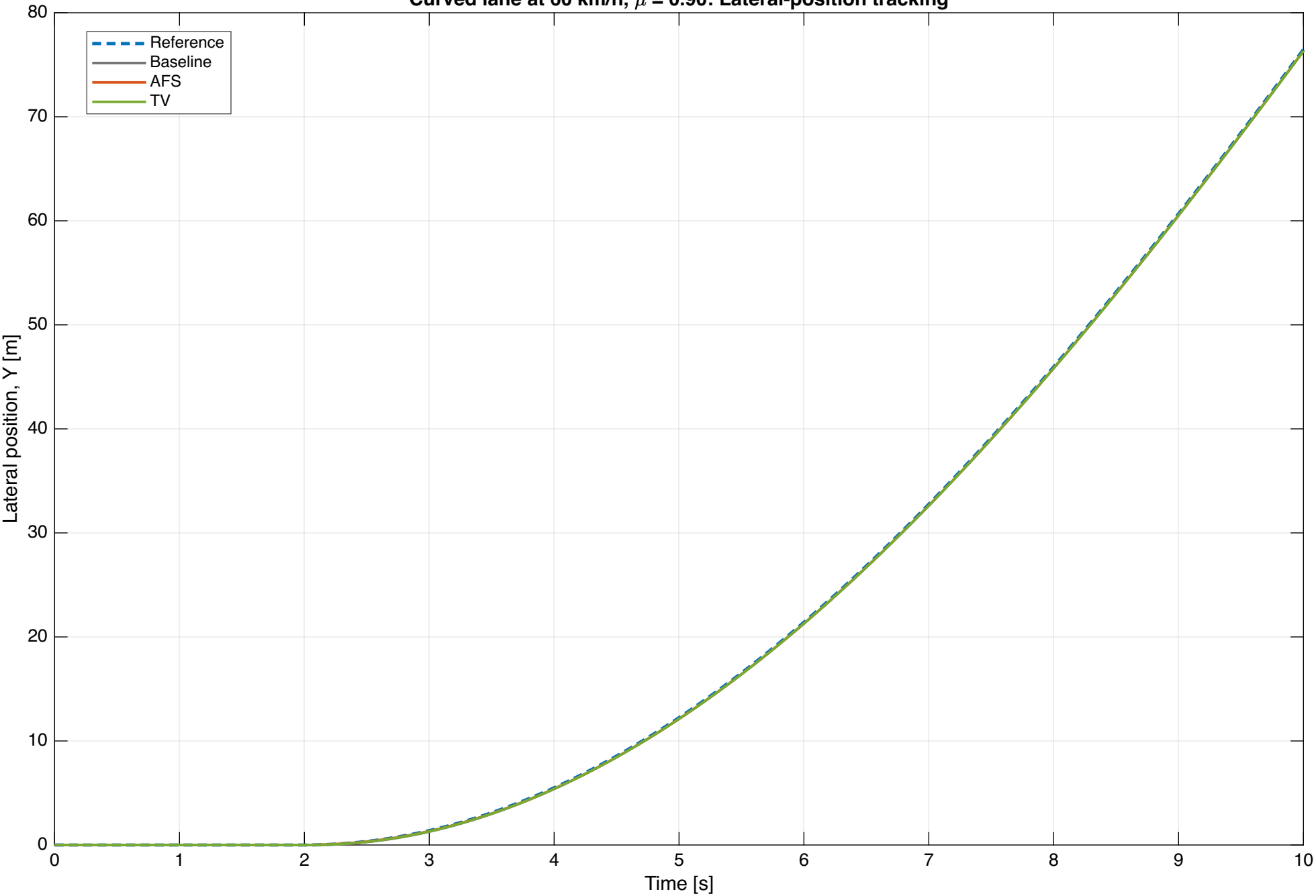
Curved lane at 60 km/h, \mu = 0.90 : Lateral-position tracking
