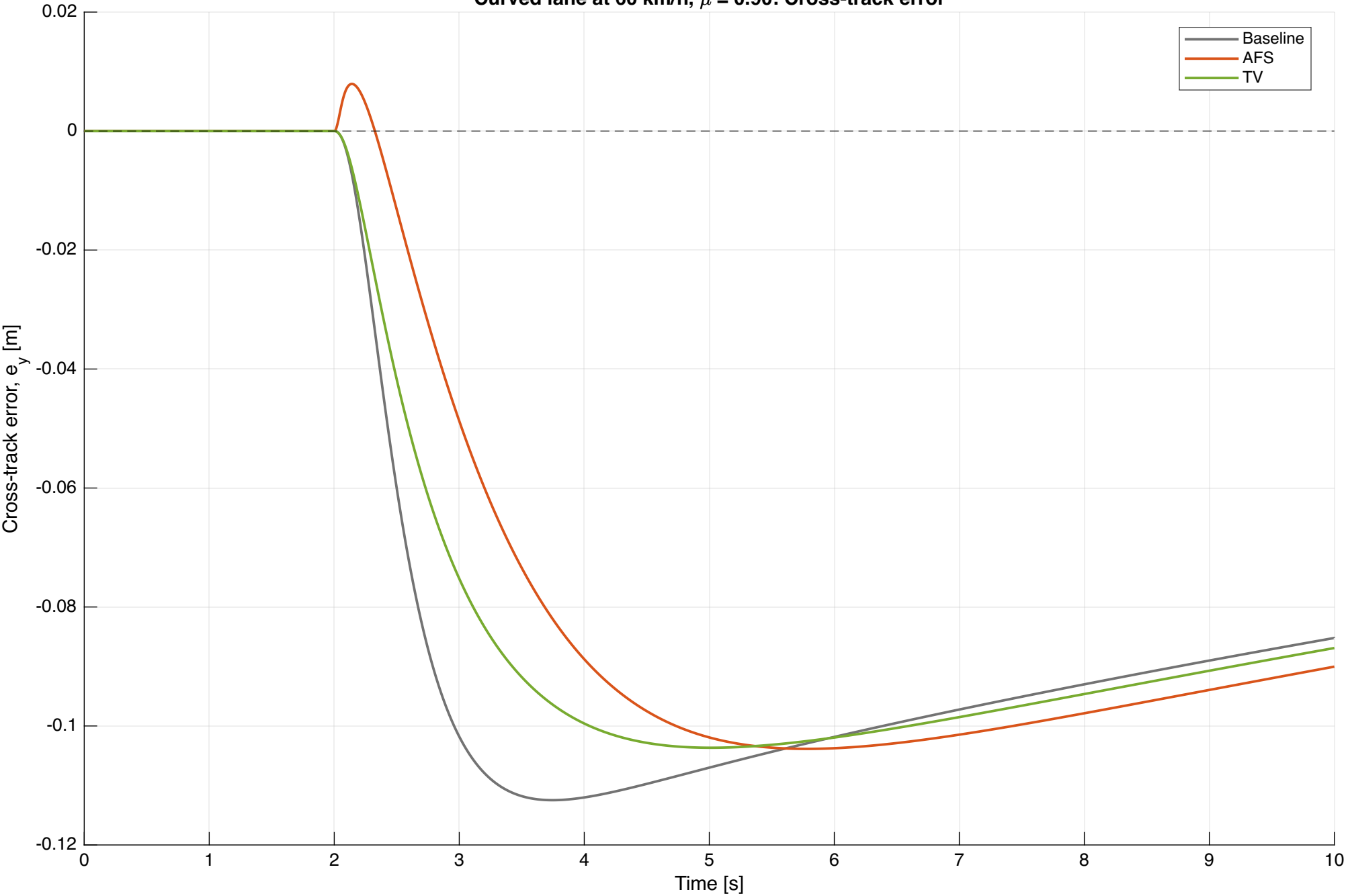
Curved lane at 60 km/h, \mu = 0.90 : Cross-track error
