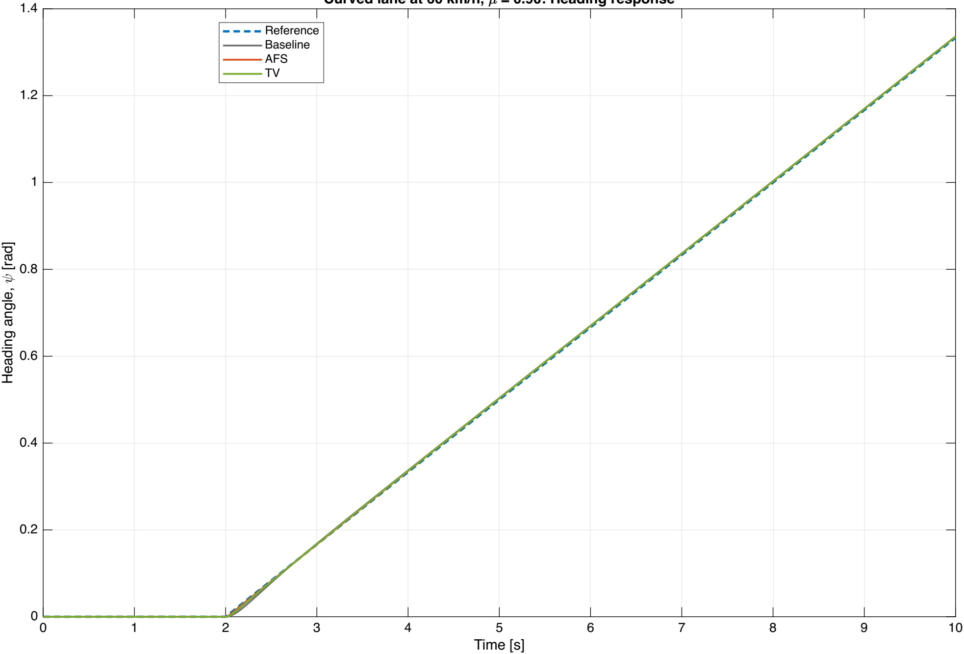
Curved lane at 60 km/h, \mu = 0.90 : Heading response
