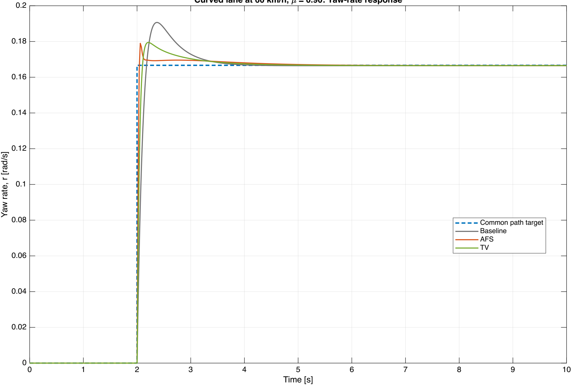
Curved lane at 60 km/h, \mu = 0.90 : Yaw-rate response
