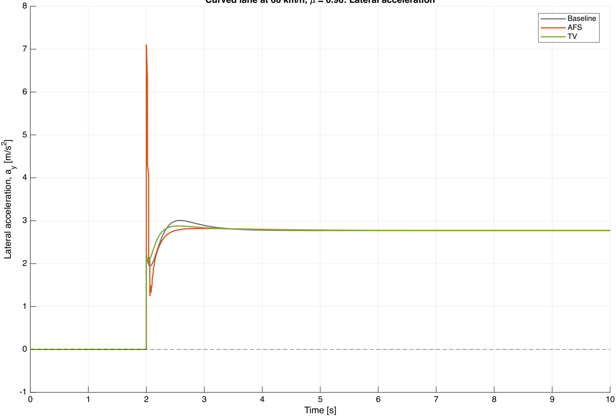
Curved lane at 60 km/h, \mu = 0.90 : Lateral acceleration
