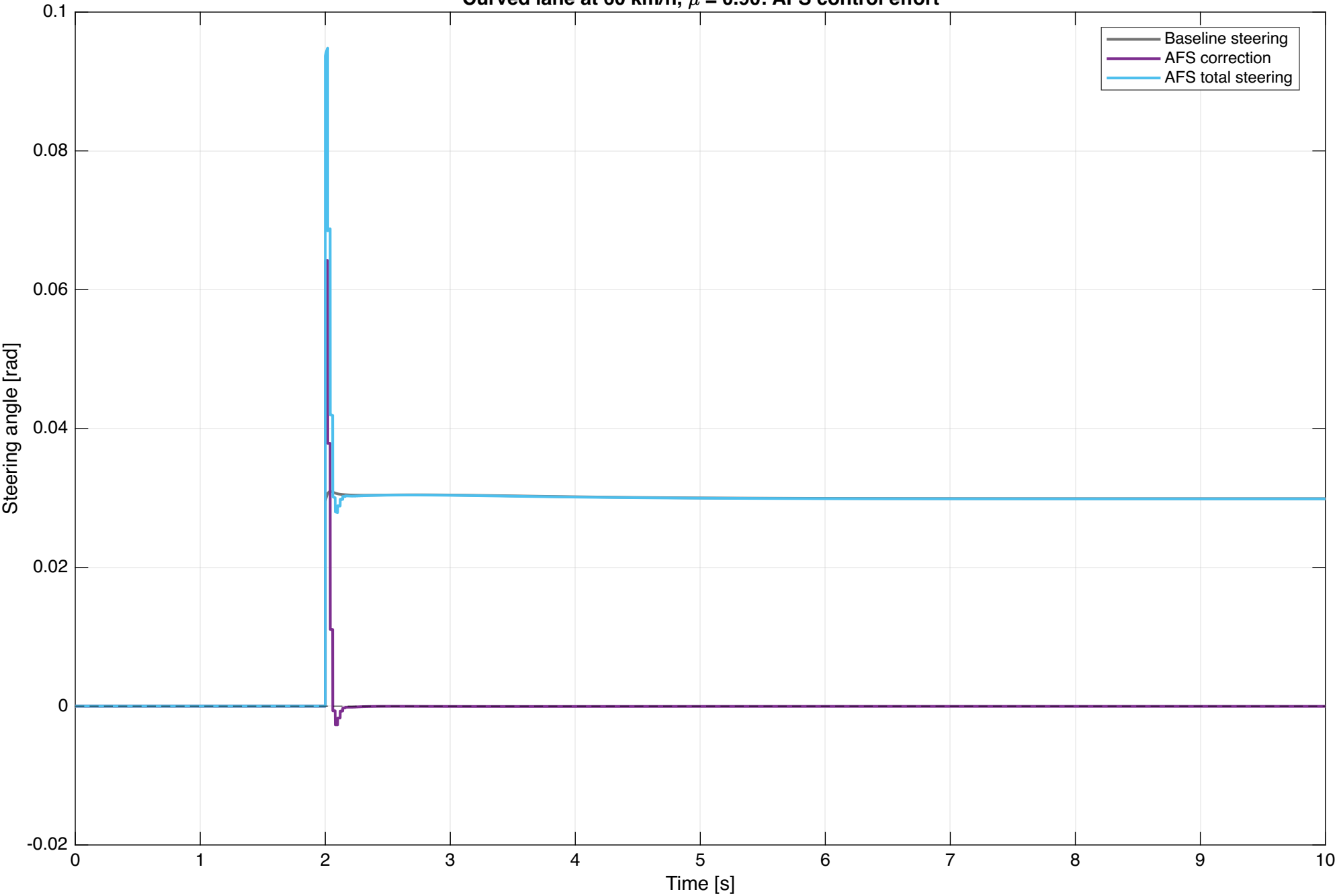
Curved lane at 60 km/h, \mu = 0.90 : AFS control effort
