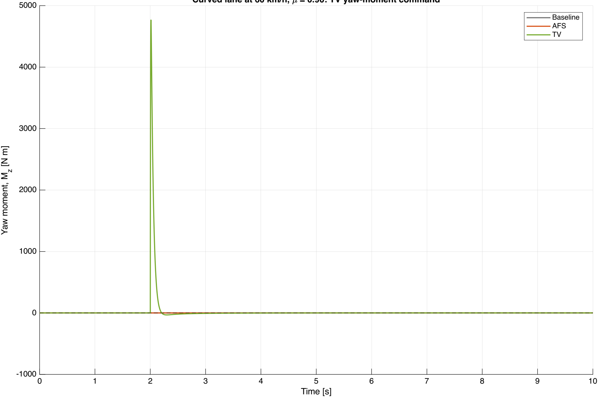
Curved lane at 60 km/h, \mu = 0.90 : TV yaw-moment command
