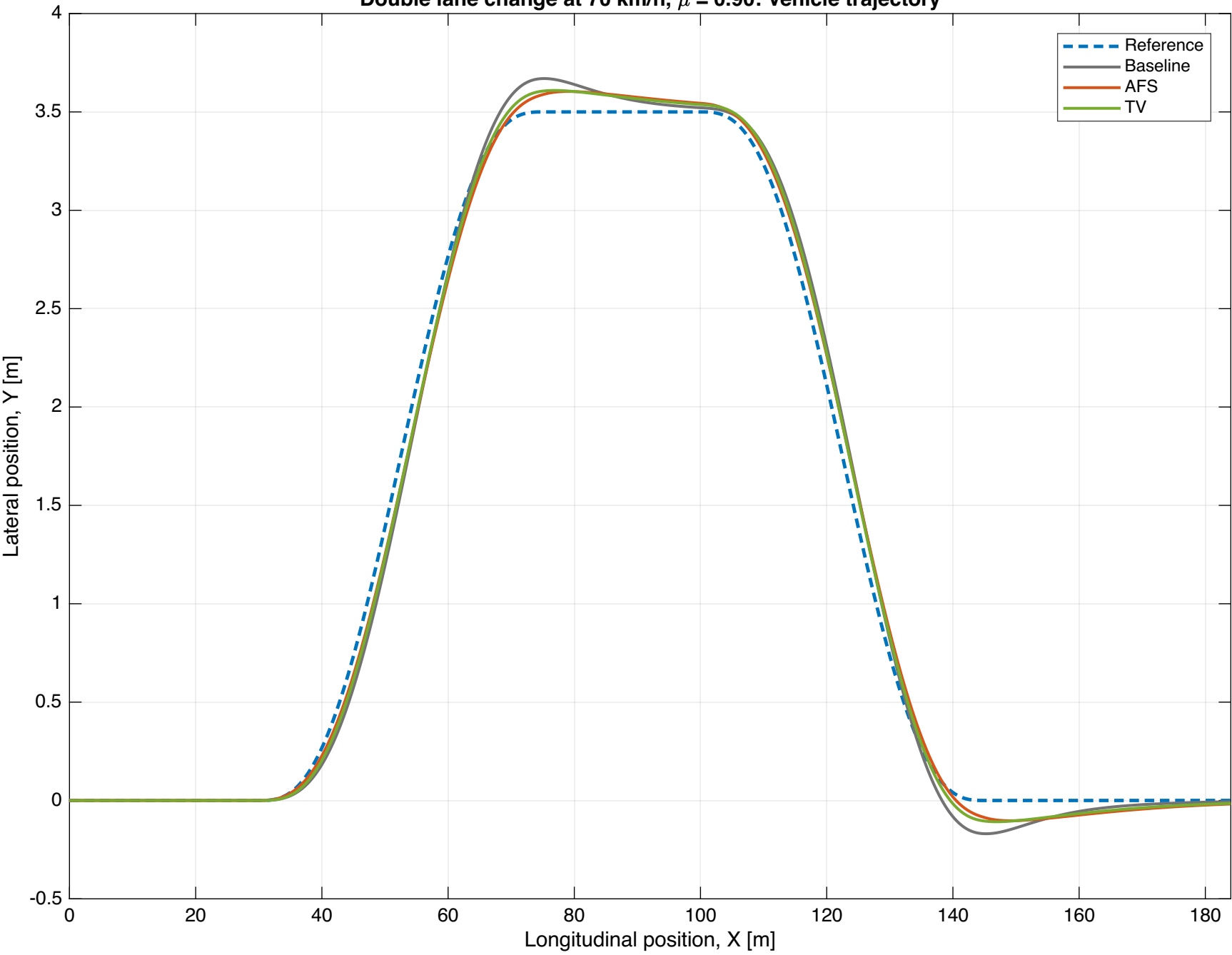
Double lane change at 70 km/h, \mu = 0.90 : Vehicle trajectory
