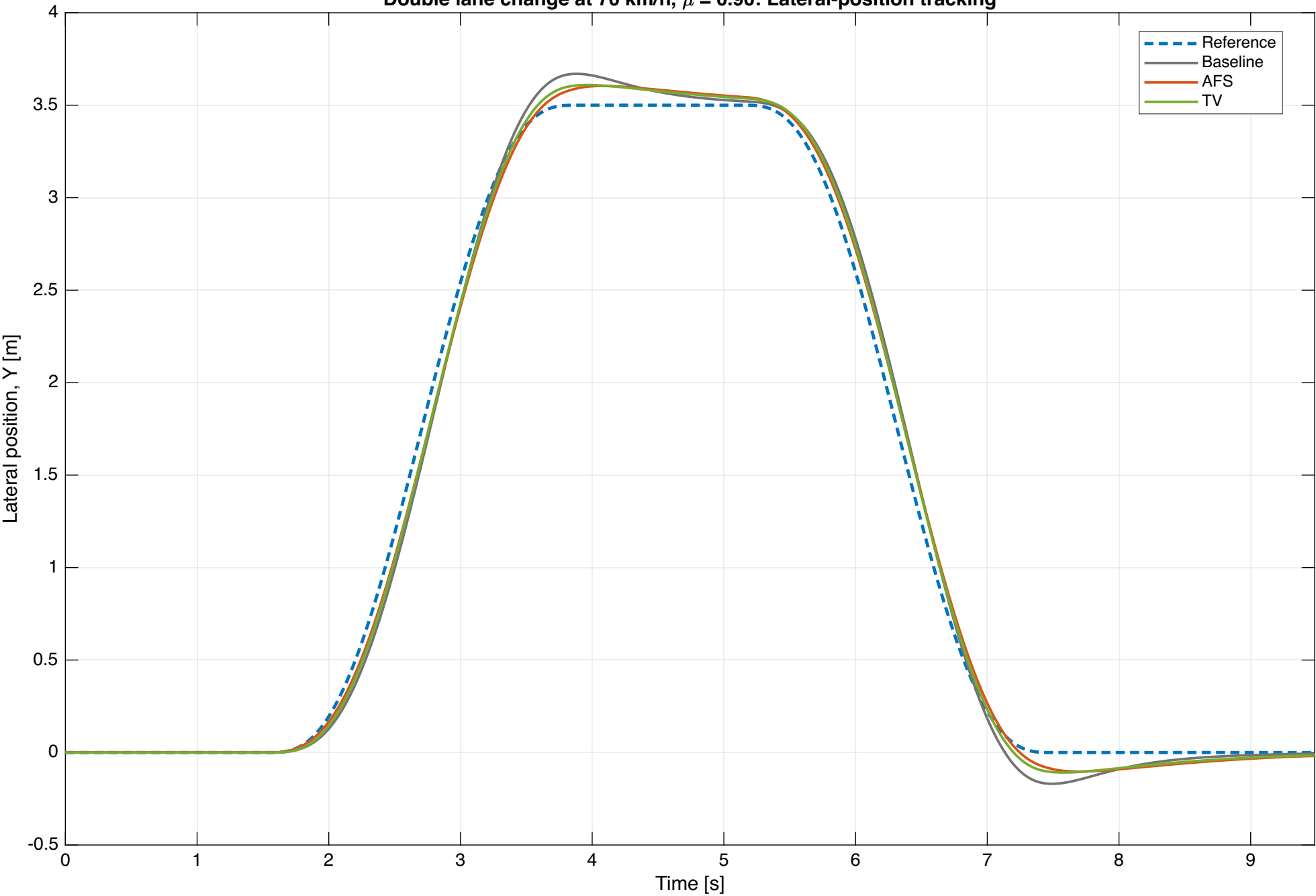
Double lane change at 70 km/h, \mu = 0.90 : Lateral-position tracking
